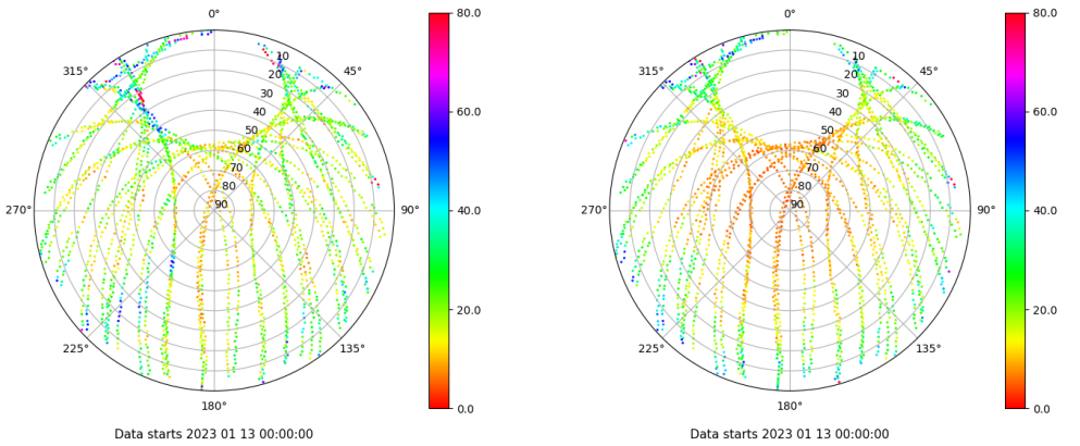
Skyplot for station SALA. Parameter M1C Data file SALA00ESP_R_2023013.xtr Skyplot for station SALA. Parameter M2P Data file SALA00ESP_R_2023013.xtr
