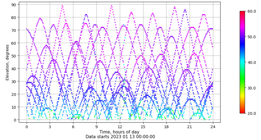
Time-elevation plot for station SALA. Signal to Noise S1C Data file SALA00ESP_R_2023013.xtr
