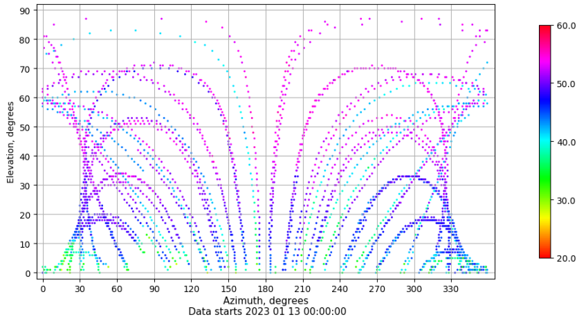
Azimuth-elevation plot for station SALA. Signal to Noise S1C Data file SALA00ESP_R_2023013.xtr
