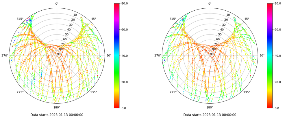
Skyplot for station SALA. Parameter M1C Data file SALA00ESP_R_2023013.xtr Skyplot for station SALA. Parameter M2S Data file SALA00ESP_R_2023013.xtr
