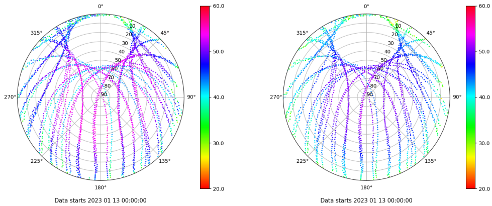
Skyplot for station SALA. Signal to Noise S1C Data file SALA00ESP_R_2023013.xtr Skyplot for station SALA. Signal to Noise S2P Data file SALA00ESP_R_2023013.xtr
