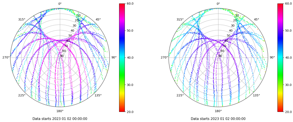
Skyplot for station SALA. Signal to Noise S1C Data file SALA00ESP_R_2023002.xtr Skyplot for station SALA. Signal to Noise S2P Data file SALA00ESP_R_2023002.xtr
