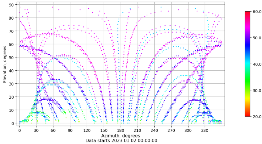
Azimuth-elevation plot for station SALA. Signal to Noise S1C Data file SALA00ESP_R_2023002.xtr
