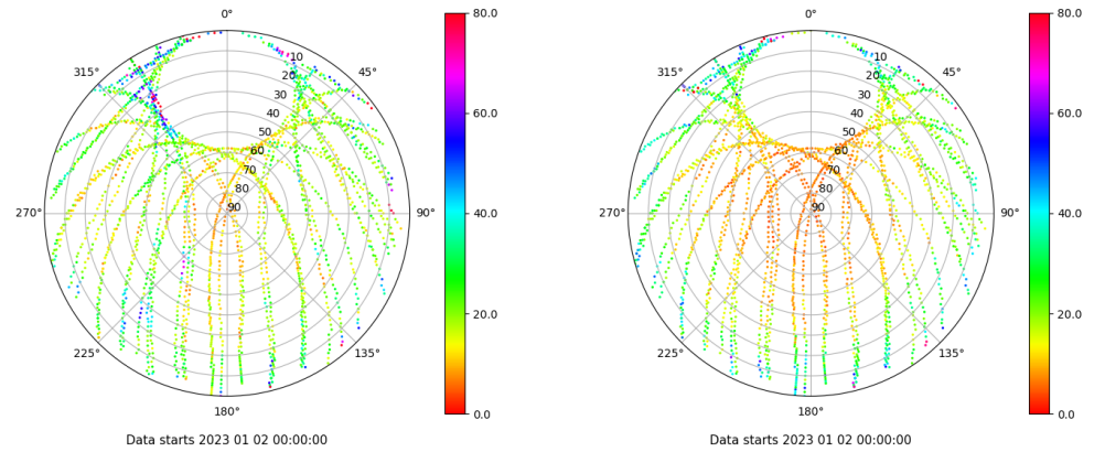
Skyplot for station SALA. Parameter M1C Data file SALA00ESP_R_2023002.xtr Skyplot for station SALA. Parameter M2P Data file SALA00ESP_R_2023002.xtr
