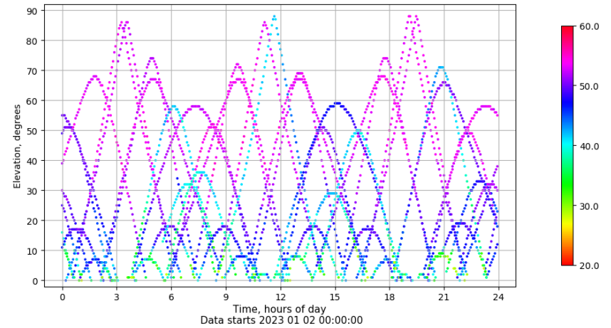
Time-elevation plot for station SALA. Signal to Noise S1C Data file SALA00ESP_R_2023002.xtr
