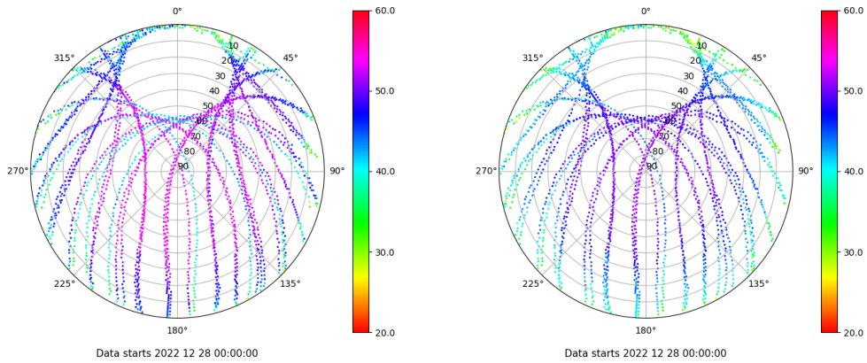
Skyplot for station SALA. Signal to Noise S1C Data file SALA00ESP_R_2022362.xtr Skyplot for station SALA. Signal to Noise S2P Data file SALA00ESP_R_2022362.xtr
