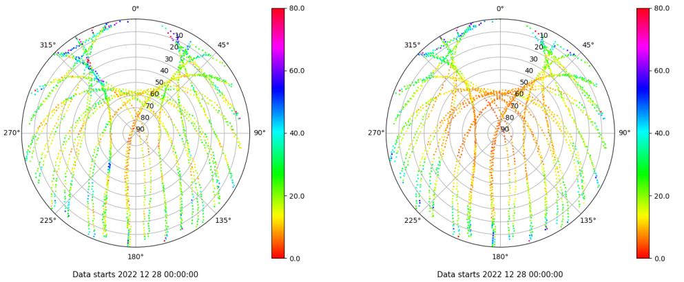
Skyplot for station SALA. Parameter M1C Data file SALA00ESP_R_2022362.xtr Skyplot for station SALA. Parameter M2P Data file SALA00ESP_R_2022362.xtr
