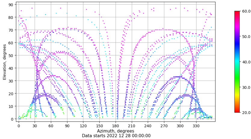
Azimuth-elevation plot for station SALA. Signal to Noise S1C Data file SALA00ESP_R_2022362.xtr
