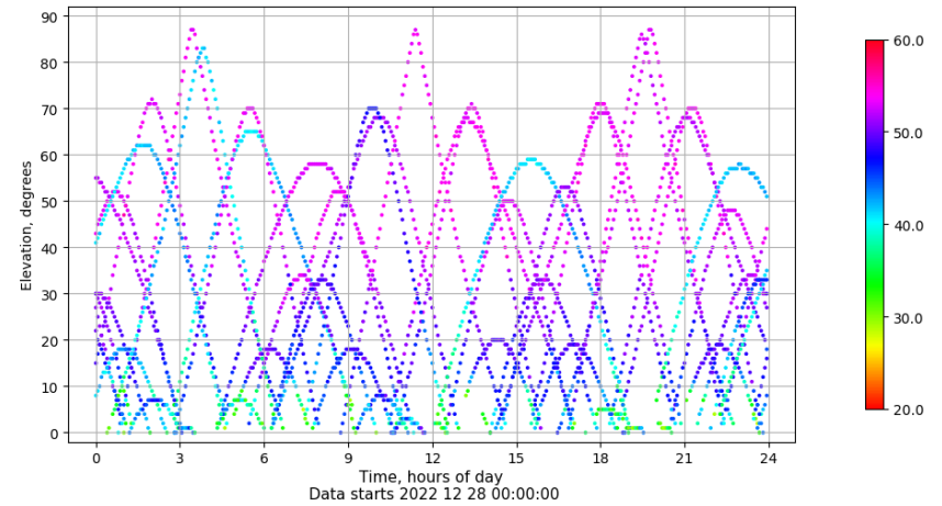
Time-elevation plot for station SALA. Signal to Noise S1C Data file SALA00ESP_R_2022362.xtr
