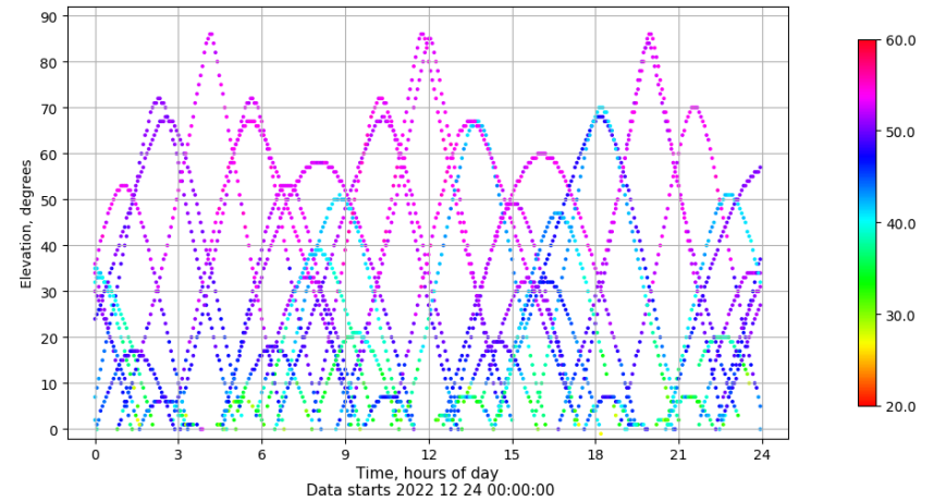
Time-elevation plot for station SALA. Signal to Noise S1C Data file SALA00ESP_R_2022358.xtr
