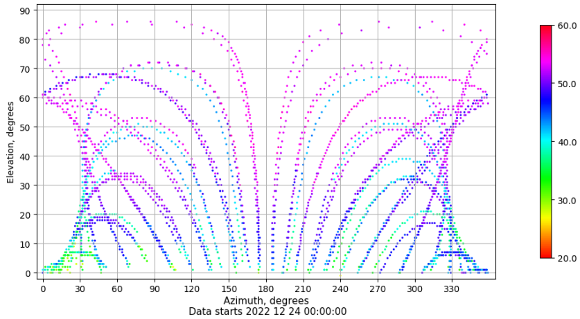
Azimuth-elevation plot for station SALA. Signal to Noise S1C Data file SALA00ESP_R_2022358.xtr
