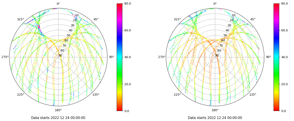
Skyplot for station SALA. Parameter M1C Data file SALA00ESP_R_2022358.xtr Skyplot for station SALA. Parameter M2P Data file SALA00ESP_R_2022358.xtr
