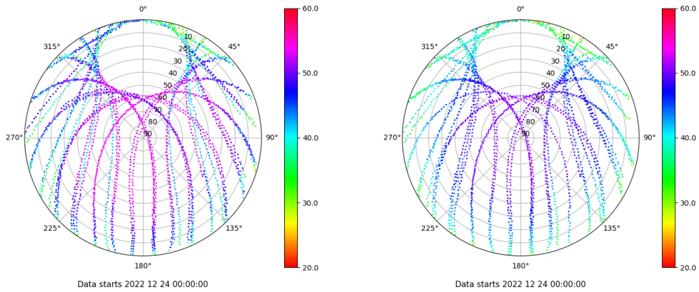
Skyplot for station SALA. Signal to Noise S1C Data file SALA00ESP_R_2022358.xtr Skyplot for station SALA. Signal to Noise S2P Data file SALA00ESP_R_2022358.xtr
