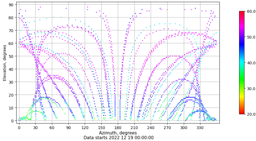
Azimuth-elevation plot for station SALA. Signal to Noise S1C Data file SALA00ESP_R_2022353.xtr
