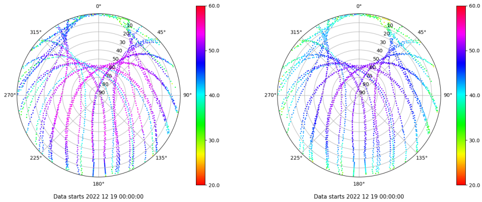
Skyplot for station SALA. Signal to Noise S1C Data file SALA00ESP_R_2022353.xtr Skyplot for station SALA. Signal to Noise S2P Data file SALA00ESP_R_2022353.xtr
