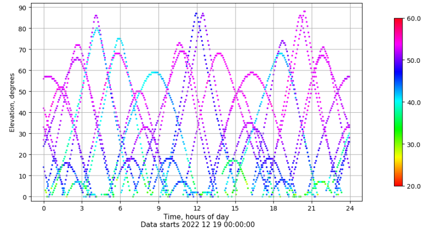
Time-elevation plot for station SALA. Signal to Noise S1C Data file SALA00ESP_R_2022353.xtr
