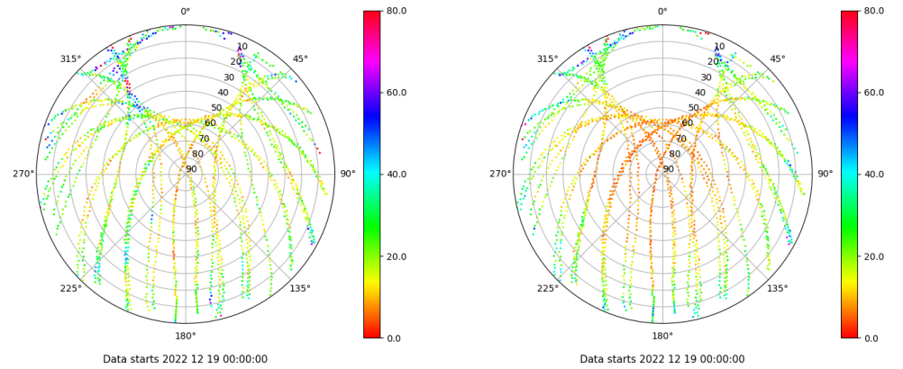
Skyplot for station SALA. Parameter M1C Data file SALA00ESP_R_2022353.xtr Skyplot for station SALA. Parameter M2P Data file SALA00ESP_R_2022353.xtr
