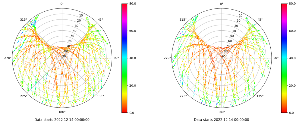
Skyplot for station SALA. Parameter M1C Data file SALA00ESP_R_2022348.xtr Skyplot for station SALA. Parameter M2S Data file SALA00ESP_R_2022348.xtr
