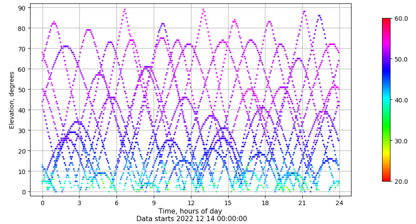
Time-elevation plot for station SALA. Signal to Noise S1C Data file SALA00ESP_R_2022348.xtr
