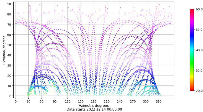
Azimuth-elevation plot for station SALA. Signal to Noise S1C Data file SALA00ESP_R_2022348.xtr
