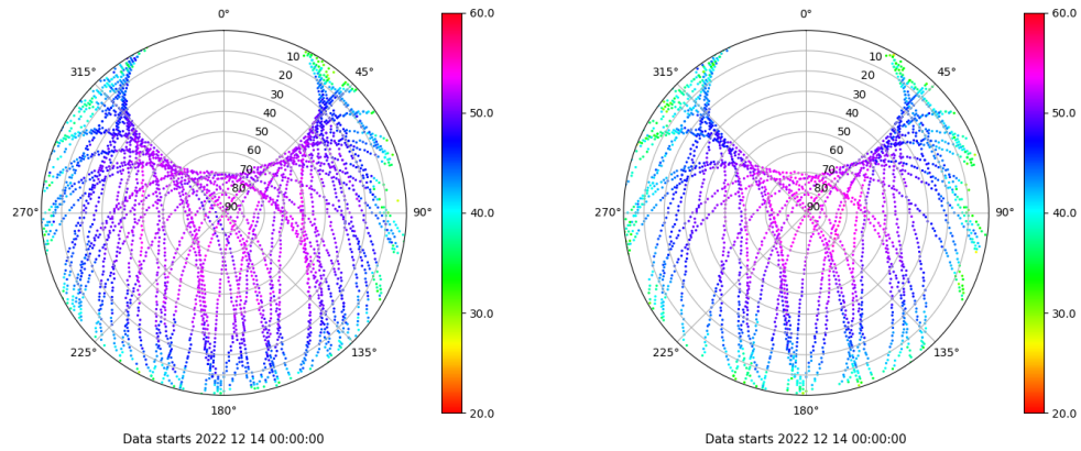
Skyplot for station SALA. Signal to Noise S1C Data file SALA00ESP_R_2022348.xtr Skyplot for station SALA. Signal to Noise S2S Data file SALA00ESP_R_2022348.xtr
