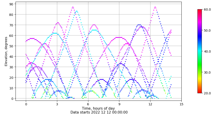
Time-elevation plot for station SALA. Signal to Noise S1C Data file SALA00ESP_R_2022346.xtr
