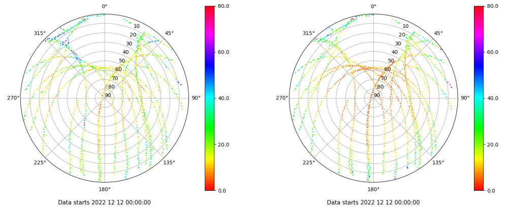
Skyplot for station SALA. Parameter M1C Data file SALA00ESP_R_2022346.xtr Skyplot for station SALA. Parameter M2P Data file SALA00ESP_R_2022346.xtr
