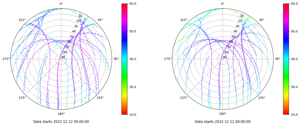
Skyplot for station SALA. Signal to Noise S1C Data file SALA00ESP_R_2022346.xtr Skyplot for station SALA. Signal to Noise S2P Data file SALA00ESP_R_2022346.xtr
