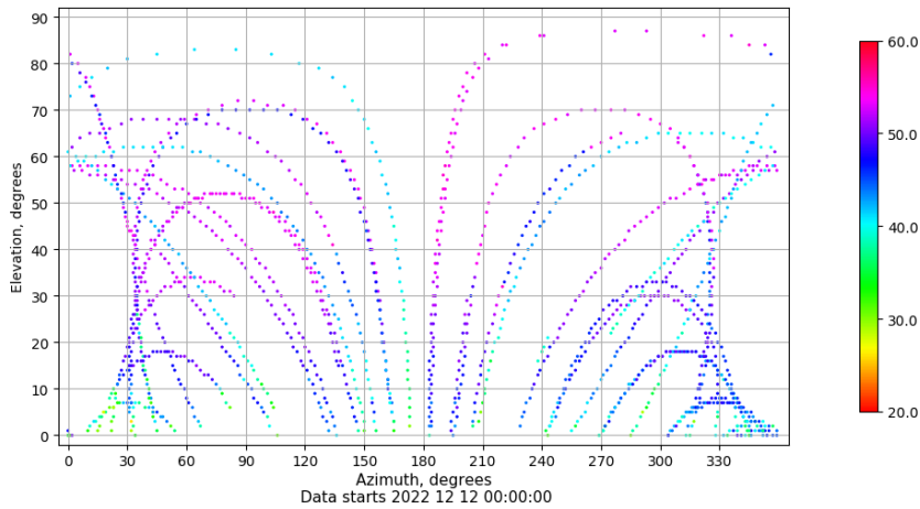
Azimuth-elevation plot for station SALA. Signal to Noise S1C Data file SALA00ESP_R_2022346.xtr
