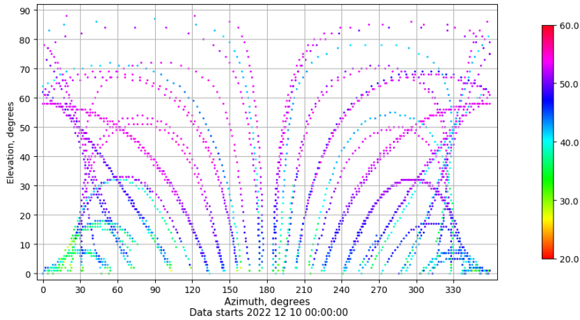
Azimuth-elevation plot for station SALA. Signal to Noise S1C Data file SALA00ESP_R_2022344.xtr
