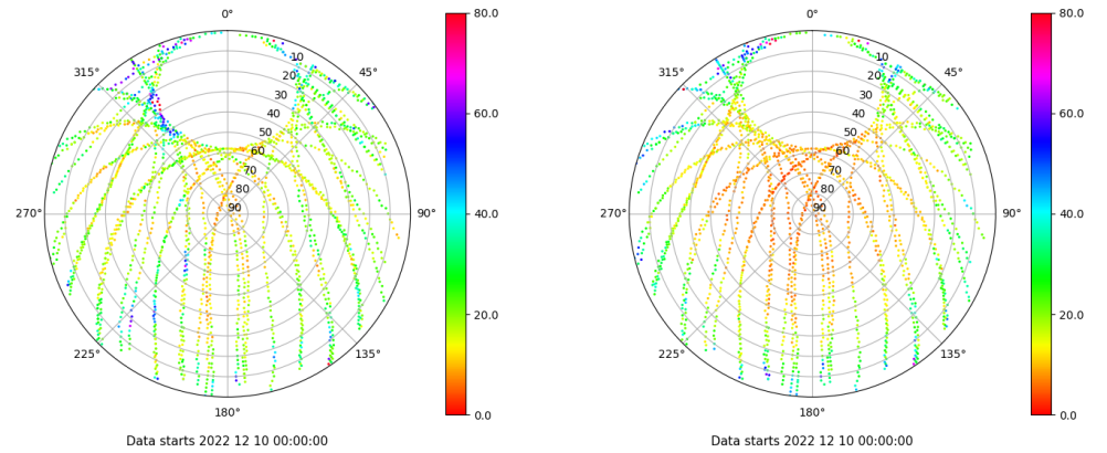
Skyplot for station SALA. Parameter M1C Data file SALA00ESP_R_2022344.xtr Skyplot for station SALA. Parameter M2P Data file SALA00ESP_R_2022344.xtr
