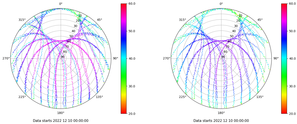
Skyplot for station SALA. Signal to Noise S1C Data file SALA00ESP_R_2022344.xtr Skyplot for station SALA. Signal to Noise S2P Data file SALA00ESP_R_2022344.xtr
