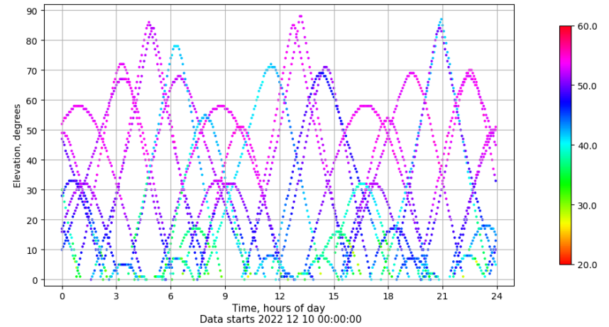
Time-elevation plot for station SALA. Signal to Noise S1C Data file SALA00ESP_R_2022344.xtr
