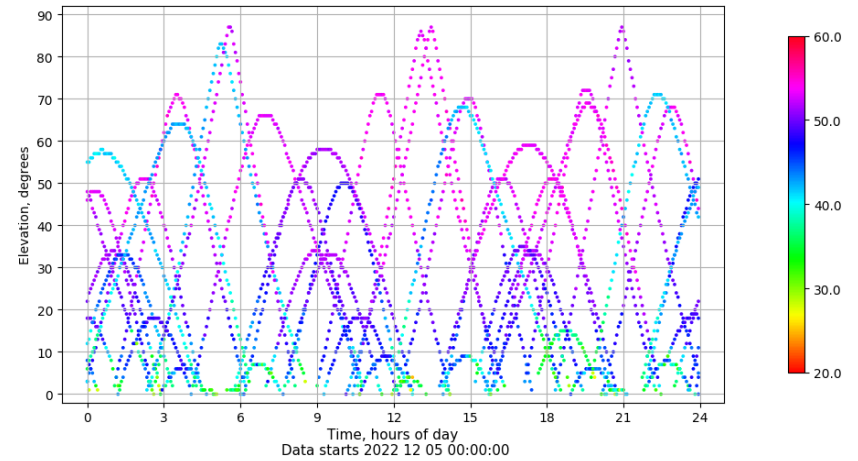
Time-elevation plot for station SALA. Signal to Noise S1C Data file SALA00ESP_R_2022339.xtr
