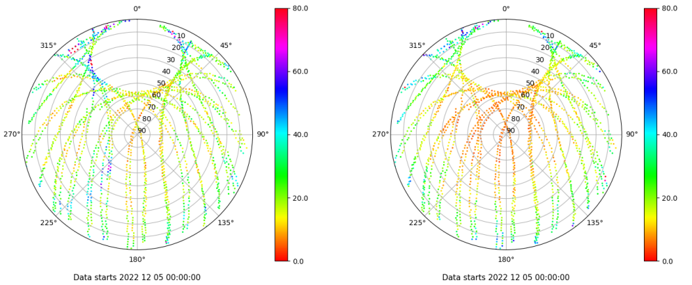
Skyplot for station SALA. Parameter M1C Data file SALA00ESP_R_2022339.xtr Skyplot for station SALA. Parameter M2P Data file SALA00ESP_R_2022339.xtr
