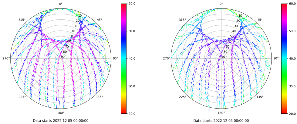
Skyplot for station SALA. Signal to Noise S1C Data file SALA00ESP_R_2022339.xtr Skyplot for station SALA. Signal to Noise S2P Data file SALA00ESP_R_2022339.xtr
