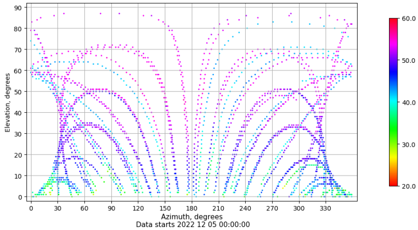
Azimuth-elevation plot for station SALA. Signal to Noise S1C Data file SALA00ESP_R_2022339.xtr
