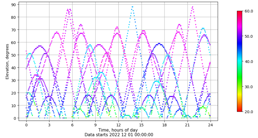
Time-elevation plot for station SALA. Signal to Noise S1C Data file SALA00ESP_R_2022335.xtr
