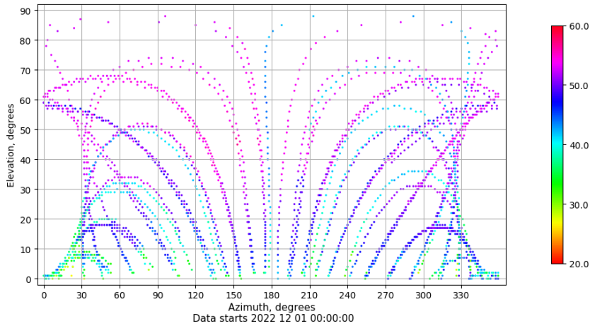
Azimuth-elevation plot for station SALA. Signal to Noise S1C Data file SALA00ESP_R_2022335.xtr
