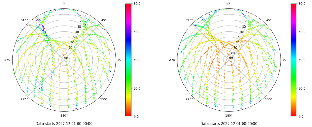
Skyplot for station SALA. Parameter M1C Data file SALA00ESP_R_2022335.xtr Skyplot for station SALA. Parameter M2P Data file SALA00ESP_R_2022335.xtr
