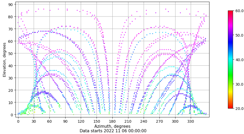
Azimuth-elevation plot for station SALA. Signal to Noise S1C Data file SALA00ESP_R_2022310.xtr
