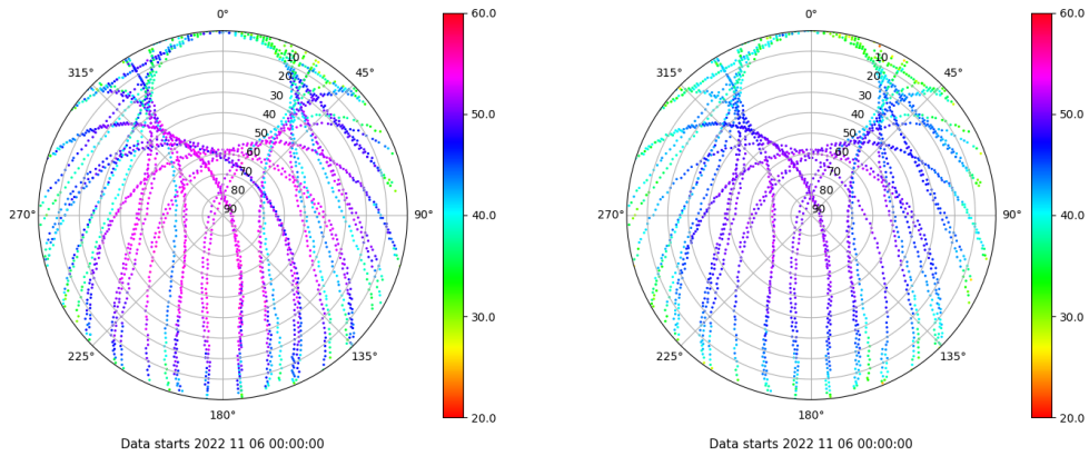
Skyplot for station SALA. Signal to Noise S1C Data file SALA00ESP_R_2022310.xtr Skyplot for station SALA. Signal to Noise S2P Data file SALA00ESP_R_2022310.xtr
