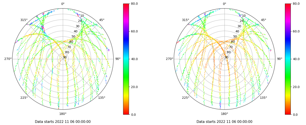
Skyplot for station SALA. Parameter M1C Data file SALA00ESP_R_2022310.xtr Skyplot for station SALA. Parameter M2P Data file SALA00ESP_R_2022310.xtr
