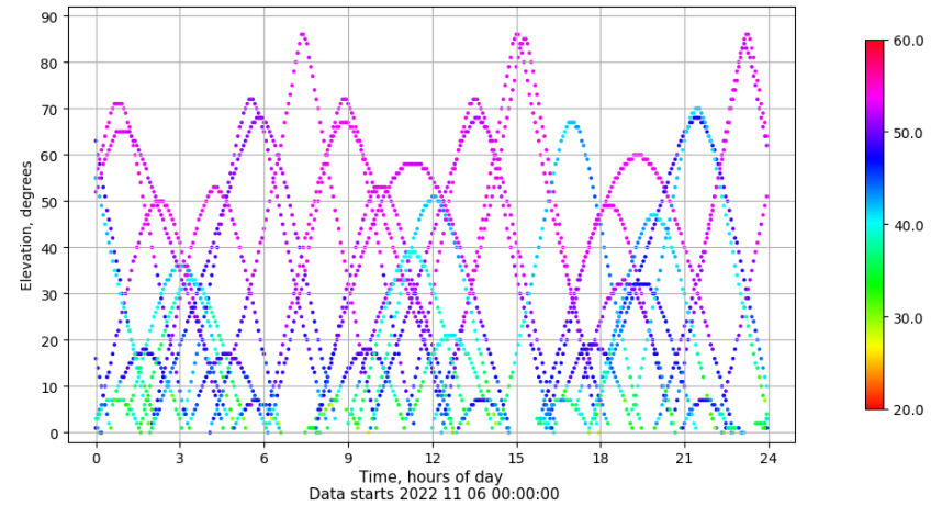
Time-elevation plot for station SALA. Signal to Noise S1C Data file SALA00ESP_R_2022310.xtr
