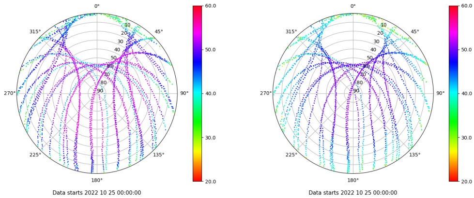
Skyplot for station SALA. Signal to Noise S1C Data file SALA00ESP_R_2022298.xtr Skyplot for station SALA. Signal to Noise S2P Data file SALA00ESP_R_2022298.xtr
