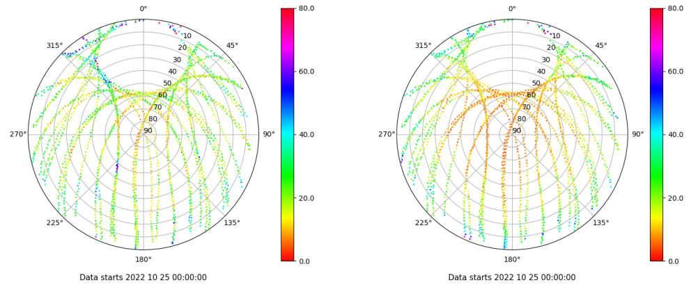
Skyplot for station SALA. Parameter M1C Data file SALA00ESP_R_2022298.xtr Skyplot for station SALA. Parameter M2P Data file SALA00ESP_R_2022298.xtr
