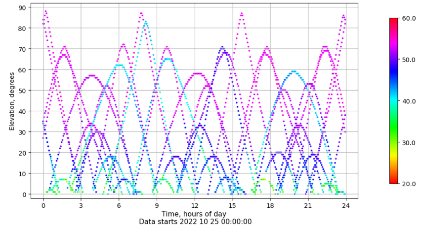
Time-elevation plot for station SALA. Signal to Noise S1C Data file SALA00ESP_R_2022298.xtr
