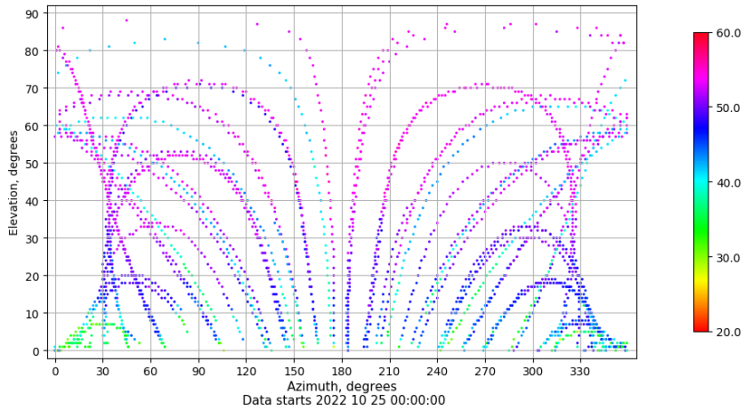
Azimuth-elevation plot for station SALA. Signal to Noise S1C Data file SALA00ESP_R_2022298.xtr
