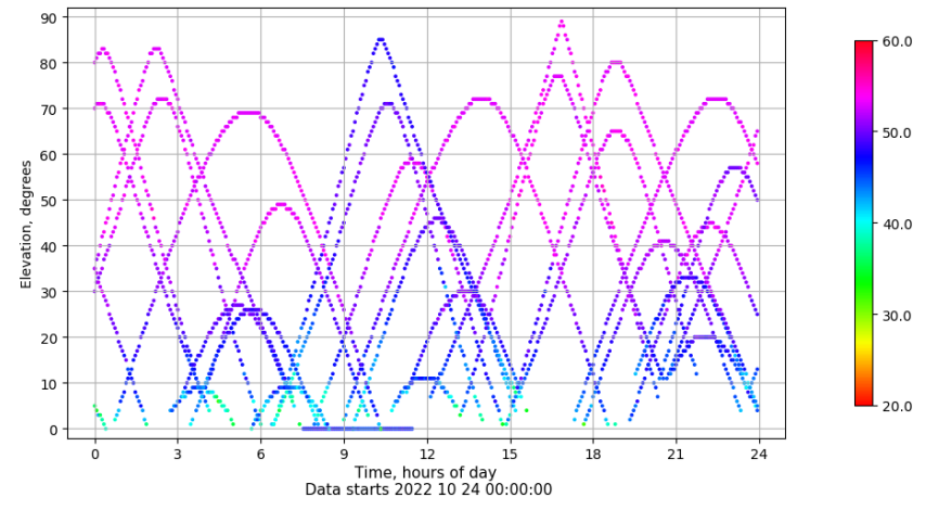
Time-elevation plot for station SALA. Signal to Noise S1C Data file SALA00ESP_R_2022297.xtr
