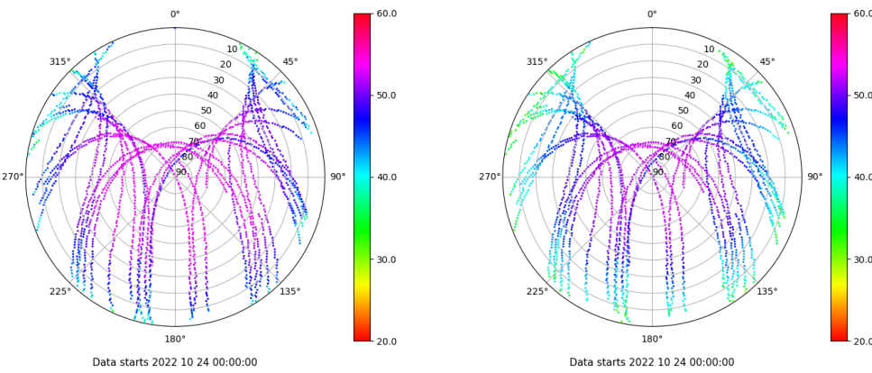
Skyplot for station SALA. Signal to Noise S1C Data file SALA00ESP_R_2022297.xtr Skyplot for station SALA. Signal to Noise S5Q Data file SALA00ESP_R_2022297.xtr
