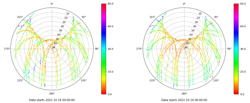
Skyplot for station SALA. Parameter M1C Data file SALA00ESP_R_2022297.xtr Skyplot for station SALA. Parameter M5Q Data file SALA00ESP_R_2022297.xtr
