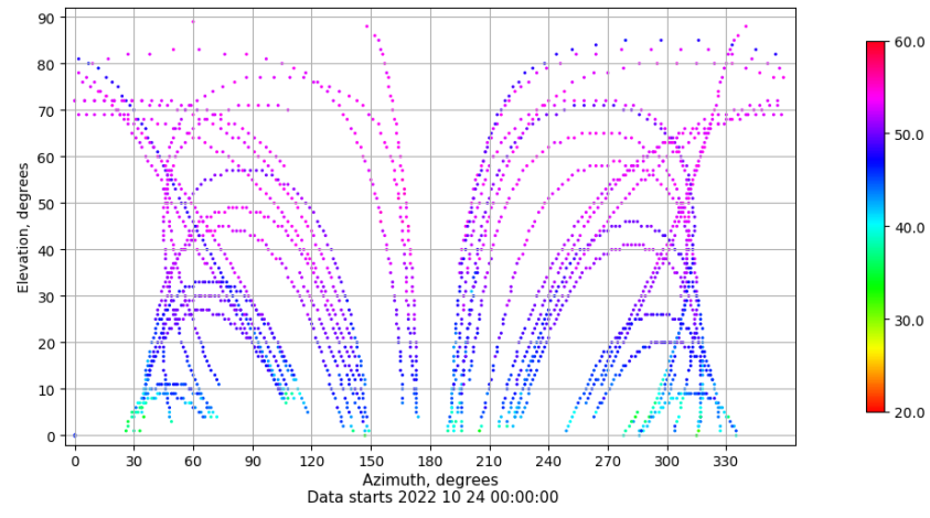
Azimuth-elevation plot for station SALA. Signal to Noise S1C Data file SALA00ESP_R_2022297.xtr
