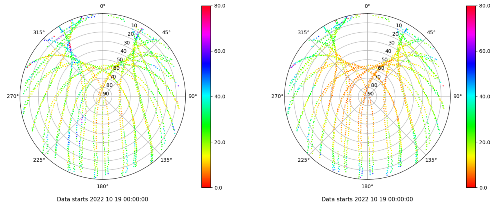
Skyplot for station SALA. Parameter M1C Data file SALA00ESP_R_2022292.xtr Skyplot for station SALA. Parameter M2P Data file SALA00ESP_R_2022292.xtr
