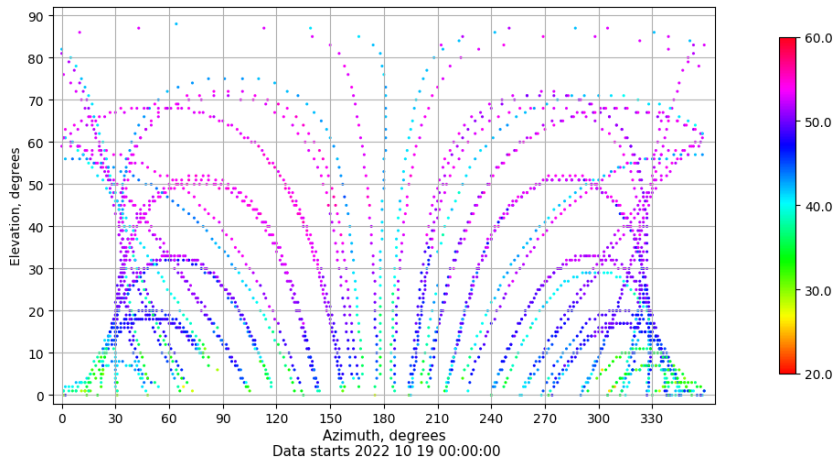
Azimuth-elevation plot for station SALA. Signal to Noise S1C Data file SALA00ESP_R_2022292.xtr
