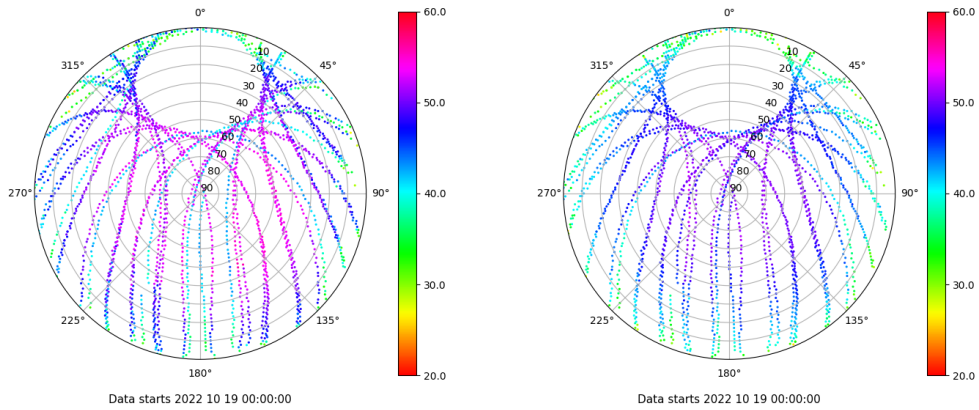
Skyplot for station SALA. Signal to Noise S1C Data file SALA00ESP_R_2022292.xtr Skyplot for station SALA. Signal to Noise S2P Data file SALA00ESP_R_2022292.xtr
