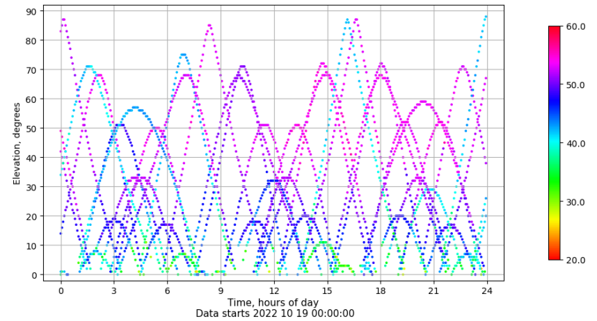
Time-elevation plot for station SALA. Signal to Noise S1C Data file SALA00ESP_R_2022292.xtr
