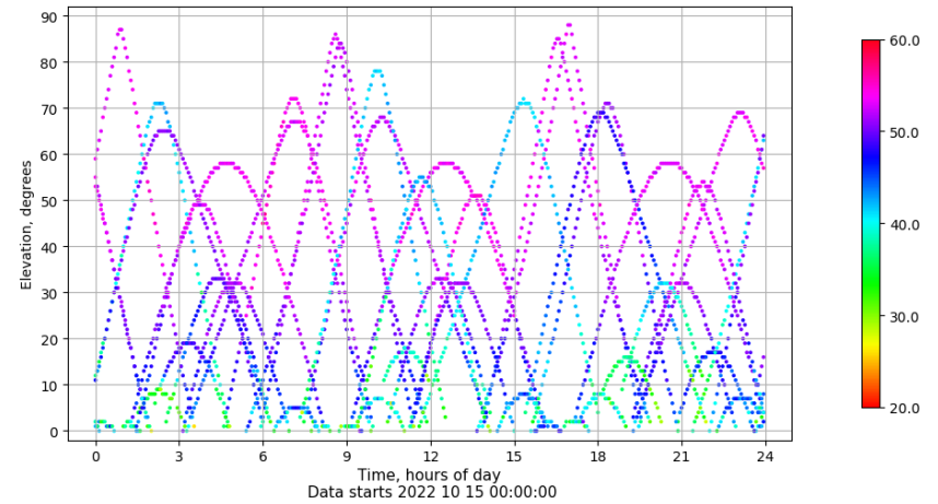
Time-elevation plot for station SALA. Signal to Noise S1C Data file SALA00ESP_R_2022288.xtr
