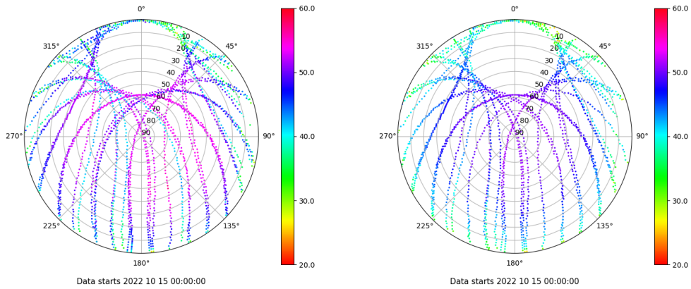
Skyplot for station SALA. Signal to Noise S1C Data file SALA00ESP_R_2022288.xtr Skyplot for station SALA. Signal to Noise S2P Data file SALA00ESP_R_2022288.xtr
