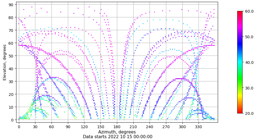
Azimuth-elevation plot for station SALA. Signal to Noise S1C Data file SALA00ESP_R_2022288.xtr
