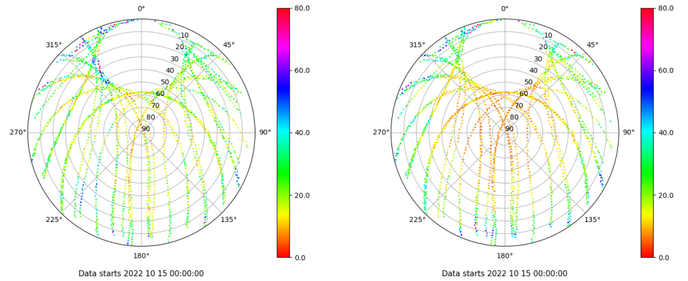
Skyplot for station SALA. Parameter M1C Data file SALA00ESP_R_2022288.xtr Skyplot for station SALA. Parameter M2P Data file SALA00ESP_R_2022288.xtr
