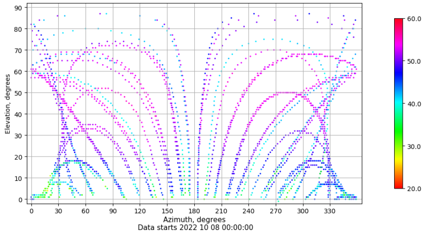
Azimuth-elevation plot for station SALA. Signal to Noise S1C Data file SALA00ESP_R_2022281.xtr
