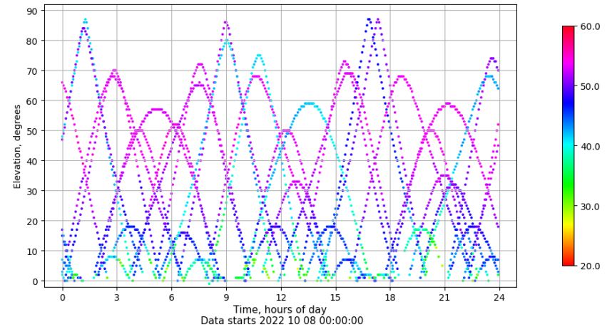
Time-elevation plot for station SALA. Signal to Noise S1C Data file SALA00ESP_R_2022281.xtr
