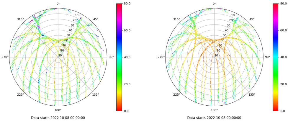
Skyplot for station SALA. Parameter M1C Data file SALA00ESP_R_2022281.xtr Skyplot for station SALA. Parameter M2P Data file SALA00ESP_R_2022281.xtr
