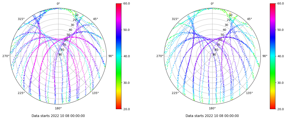
Skyplot for station SALA. Signal to Noise S1C Data file SALA00ESP_R_2022281.xtr Skyplot for station SALA. Signal to Noise S2P Data file SALA00ESP_R_2022281.xtr
