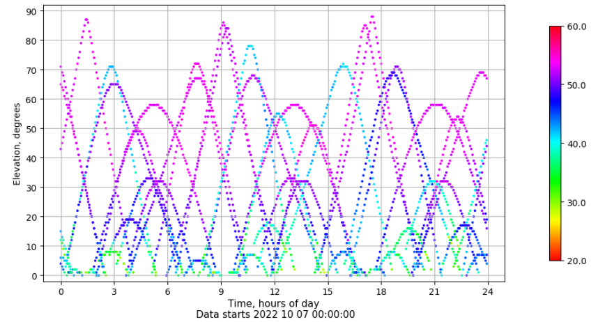
Time-elevation plot for station SALA. Signal to Noise S1C Data file SALA00ESP_R_2022280.xtr
