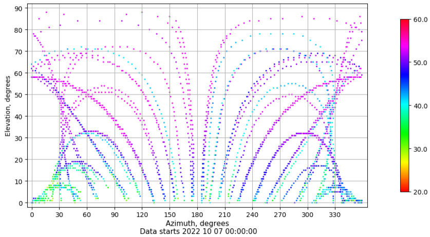
Azimuth-elevation plot for station SALA. Signal to Noise S1C Data file SALA00ESP_R_2022280.xtr
