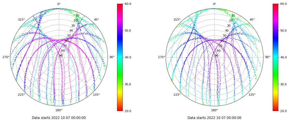
Skyplot for station SALA. Signal to Noise S1C Data file SALA00ESP_R_2022280.xtr Skyplot for station SALA. Signal to Noise S2P Data file SALA00ESP_R_2022280.xtr
