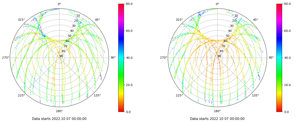
Skyplot for station SALA. Parameter M1C Data file SALA00ESP_R_2022280.xtr Skyplot for station SALA. Parameter M2P Data file SALA00ESP_R_2022280.xtr
