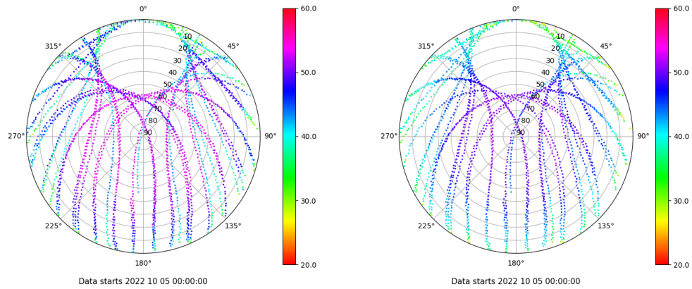
Skyplot for station SALA. Signal to Noise S1C Data file SALA00ESP_R_2022278.xtr Skyplot for station SALA. Signal to Noise S2P Data file SALA00ESP_R_2022278.xtr
