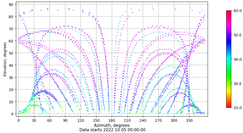
Azimuth-elevation plot for station SALA. Signal to Noise S1C Data file SALA00ESP_R_2022278.xtr
