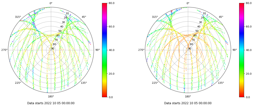
Skyplot for station SALA. Parameter M1C Data file SALA00ESP_R_2022278.xtr Skyplot for station SALA. Parameter M2P Data file SALA00ESP_R_2022278.xtr
