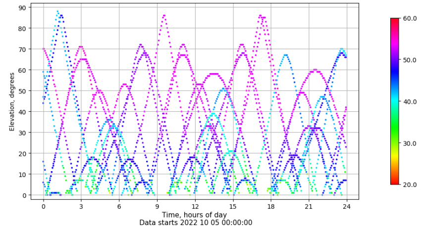
Time-elevation plot for station SALA. Signal to Noise S1C Data file SALA00ESP_R_2022278.xtr
