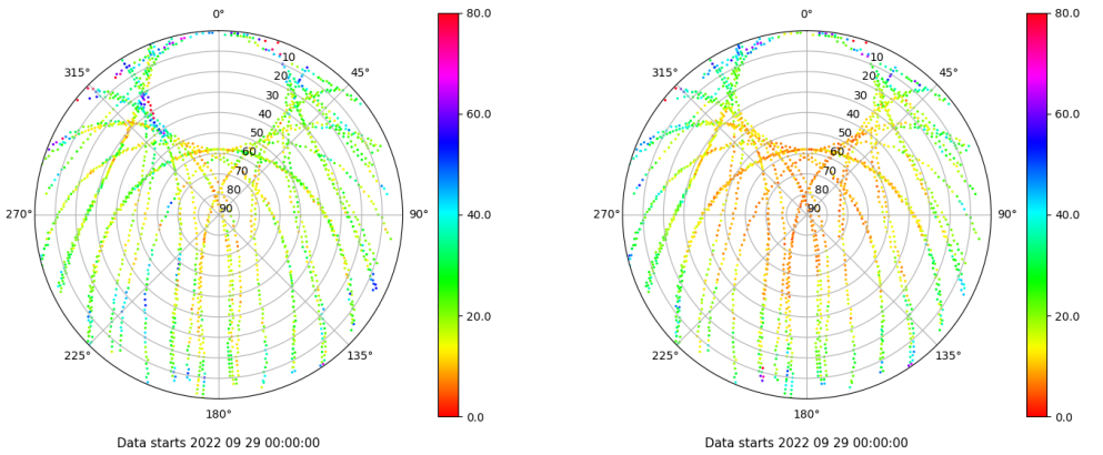
Skyplot for station SALA. Parameter M1C Data file SALA00ESP_R_2022272.xtr Skyplot for station SALA. Parameter M2P Data file SALA00ESP_R_2022272.xtr
