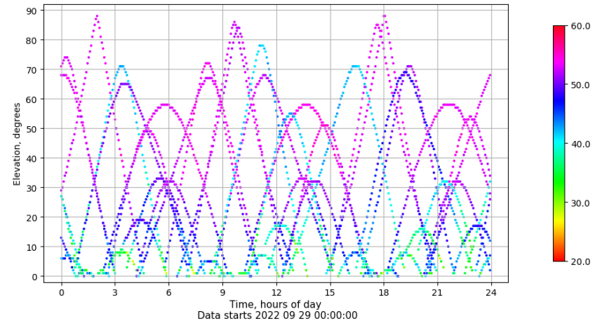
Time-elevation plot for station SALA. Signal to Noise S1C Data file SALA00ESP_R_2022272.xtr
