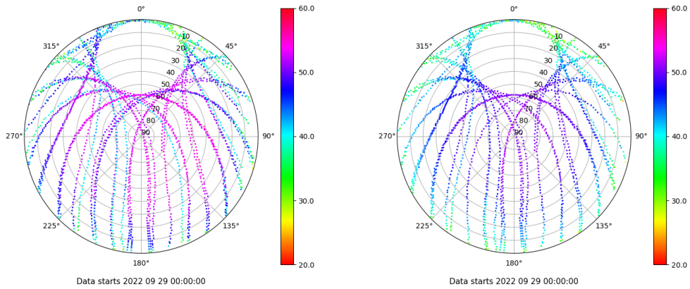
Skyplot for station SALA. Signal to Noise S1C Data file SALA00ESP_R_2022272.xtr Skyplot for station SALA. Signal to Noise S2P Data file SALA00ESP_R_2022272.xtr
