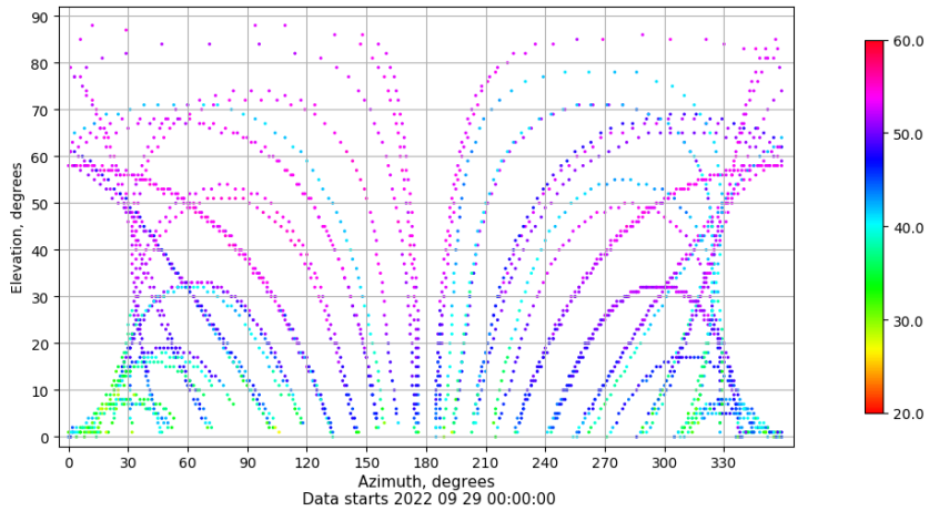
Azimuth-elevation plot for station SALA. Signal to Noise S1C Data file SALA00ESP_R_2022272.xtr
