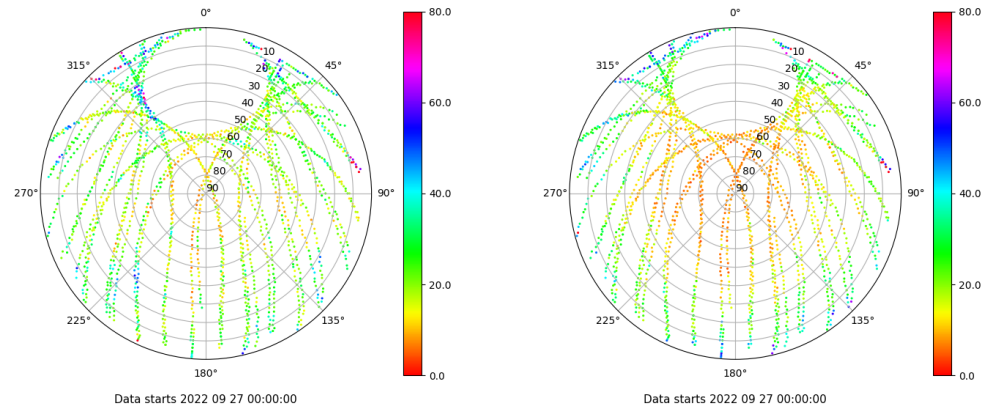
Skyplot for station SALA. Parameter M1C Data file SALA00ESP_R_2022270.xtr Skyplot for station SALA. Parameter M2P Data file SALA00ESP_R_2022270.xtr
