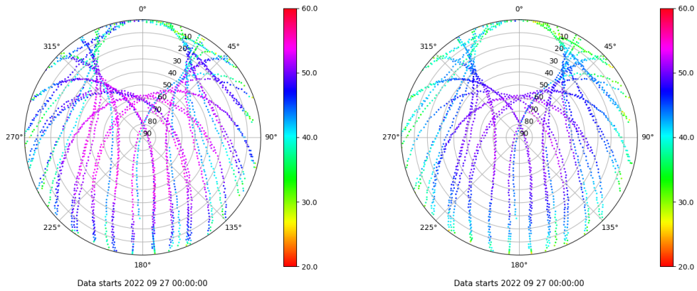
Skyplot for station SALA. Signal to Noise S1C Data file SALA00ESP_R_2022270.xtr Skyplot for station SALA. Signal to Noise S2P Data file SALA00ESP_R_2022270.xtr
