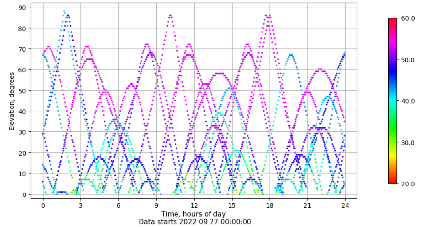
Time-elevation plot for station SALA. Signal to Noise S1C Data file SALA00ESP_R_2022270.xtr
