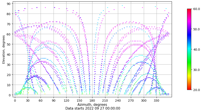
Azimuth-elevation plot for station SALA. Signal to Noise S1C Data file SALA00ESP_R_2022270.xtr
