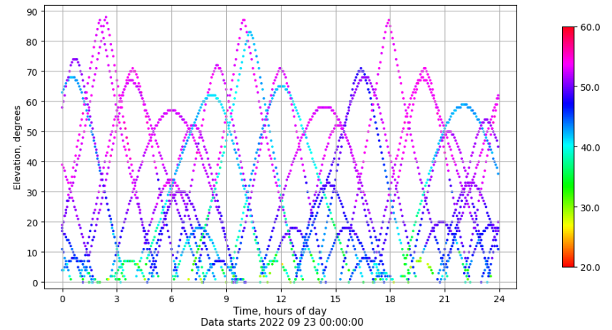
Time-elevation plot for station SALA. Signal to Noise S1C Data file SALA00ESP_R_2022266.xtr
