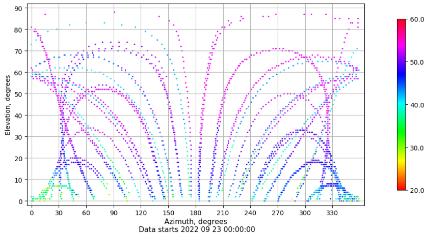
Azimuth-elevation plot for station SALA. Signal to Noise S1C Data file SALA00ESP_R_2022266.xtr
