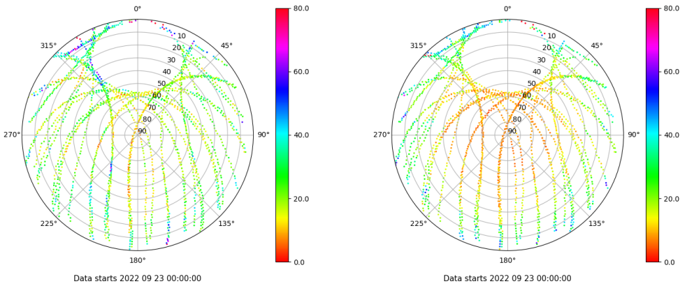
Skyplot for station SALA. Parameter M1C Data file SALA00ESP_R_2022266.xtr Skyplot for station SALA. Parameter M2P Data file SALA00ESP_R_2022266.xtr
