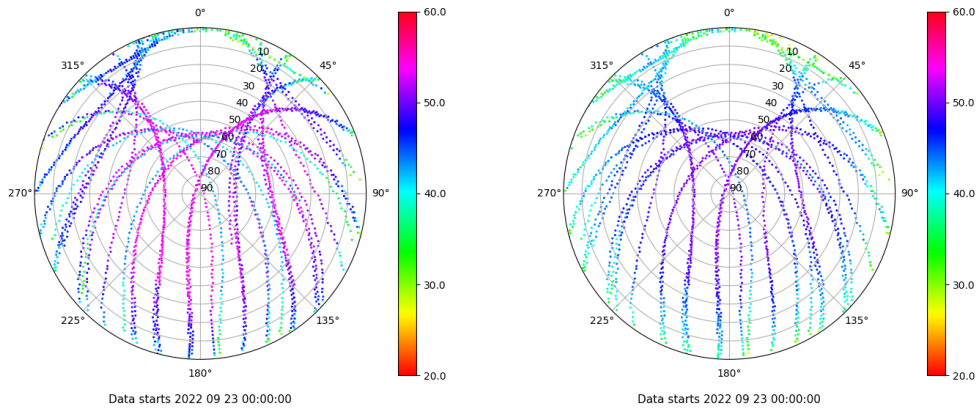
Skyplot for station SALA. Signal to Noise S1C Data file SALA00ESP_R_2022266.xtr Skyplot for station SALA. Signal to Noise S2P Data file SALA00ESP_R_2022266.xtr
