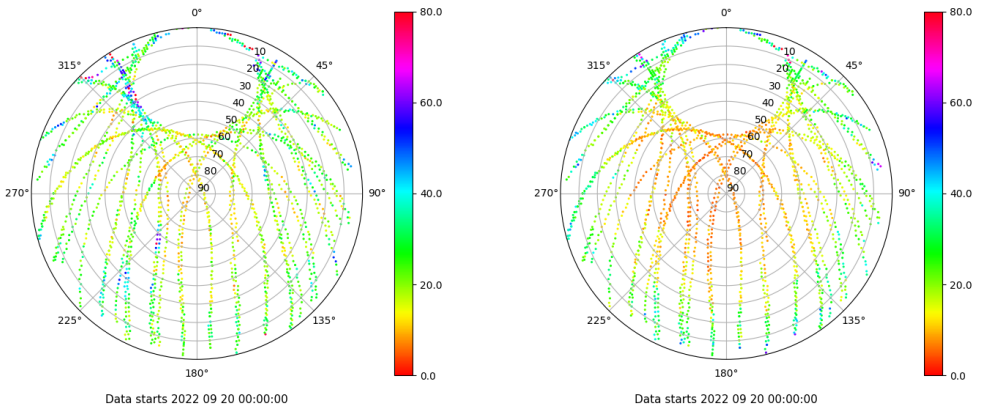
Skyplot for station SALA. Parameter M1C Data file SALA00ESP_R_2022263.xtr Skyplot for station SALA. Parameter M2P Data file SALA00ESP_R_2022263.xtr
