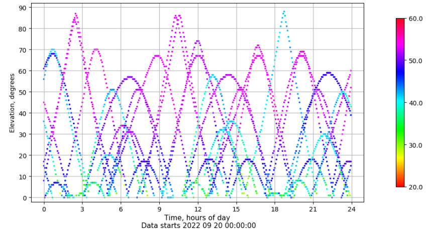
Time-elevation plot for station SALA. Signal to Noise S1C Data file SALA00ESP_R_2022263.xtr
