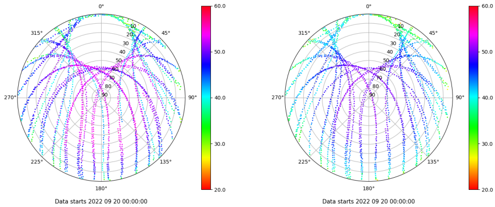
Skyplot for station SALA. Signal to Noise S1C Data file SALA00ESP_R_2022263.xtr Skyplot for station SALA. Signal to Noise S2P Data file SALA00ESP_R_2022263.xtr
