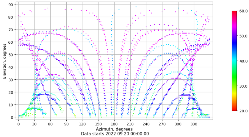
Azimuth-elevation plot for station SALA. Signal to Noise S1C Data file SALA00ESP_R_2022263.xtr
