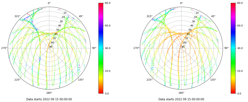
Skyplot for station SALA. Parameter M1C Data file SALA00ESP_R_2022258.xtr Skyplot for station SALA. Parameter M2P Data file SALA00ESP_R_2022258.xtr
