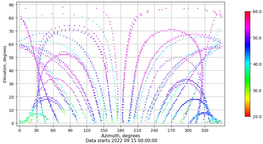
Azimuth-elevation plot for station SALA. Signal to Noise S1C Data file SALA00ESP_R_2022258.xtr
