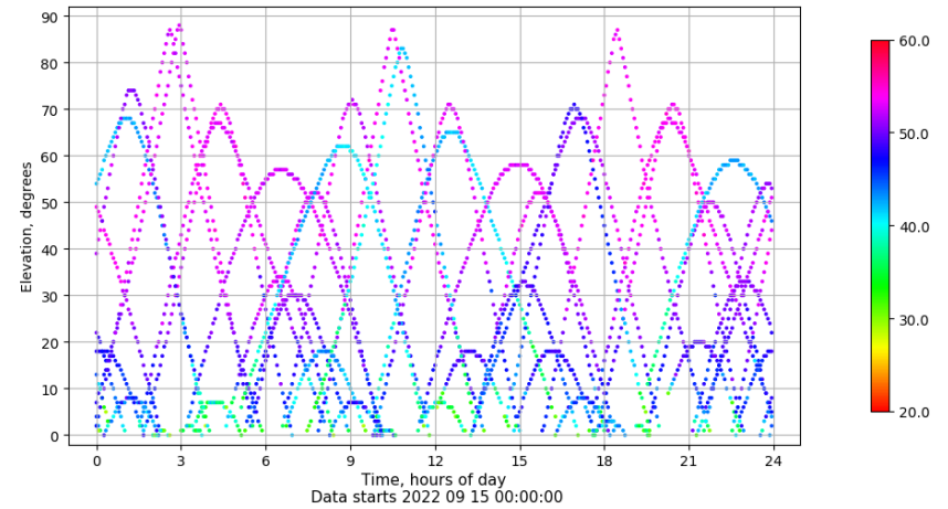
Time-elevation plot for station SALA. Signal to Noise S1C Data file SALA00ESP_R_2022258.xtr
