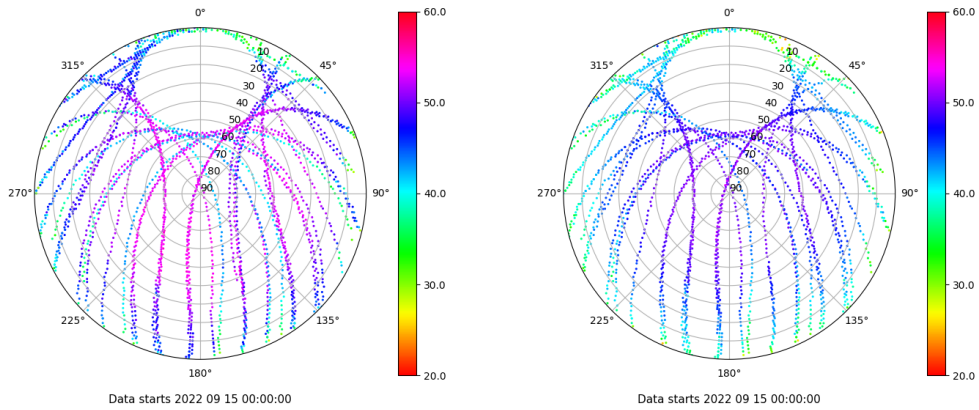
Skyplot for station SALA. Signal to Noise S1C Data file SALA00ESP_R_2022258.xtr Skyplot for station SALA. Signal to Noise S2P Data file SALA00ESP_R_2022258.xtr
