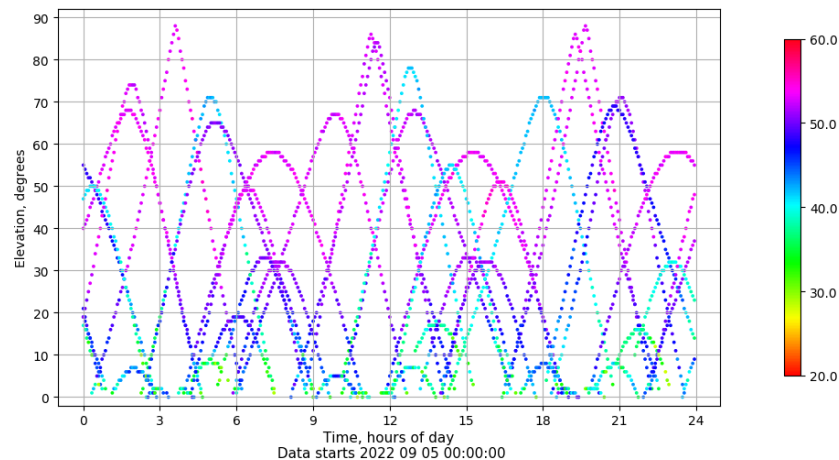
Time-elevation plot for station SALA. Signal to Noise S1C Data file SALA00ESP_R_2022248.xtr
