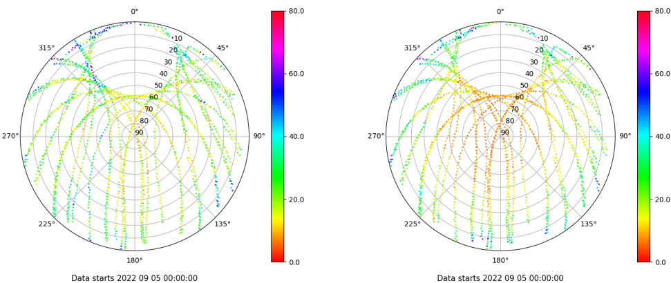
Skyplot for station SALA. Parameter M1C Data file SALA00ESP_R_2022248.xtr Skyplot for station SALA. Parameter M2P Data file SALA00ESP_R_2022248.xtr
