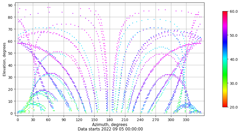
Azimuth-elevation plot for station SALA. Signal to Noise S1C Data file SALA00ESP_R_2022248.xtr
