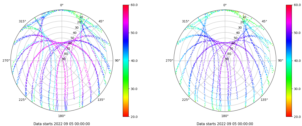
Skyplot for station SALA. Signal to Noise S1C Data file SALA00ESP_R_2022248.xtr Skyplot for station SALA. Signal to Noise S2P Data file SALA00ESP_R_2022248.xtr
