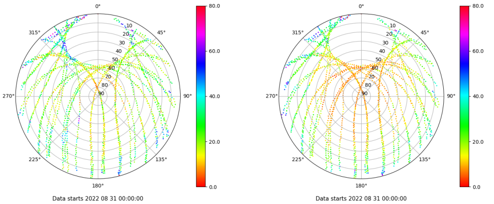
Skyplot for station SALA. Parameter M1C Data file SALA00ESP_R_2022243.xtr Skyplot for station SALA. Parameter M2P Data file SALA00ESP_R_2022243.xtr
