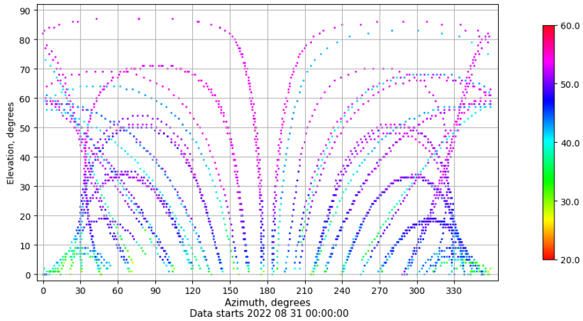
Azimuth-elevation plot for station SALA. Signal to Noise S1C Data file SALA00ESP_R_2022243.xtr
