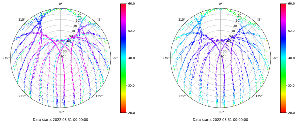
Skyplot for station SALA. Signal to Noise S1C Data file SALA00ESP_R_2022243.xtr Skyplot for station SALA. Signal to Noise S2P Data file SALA00ESP_R_2022243.xtr
