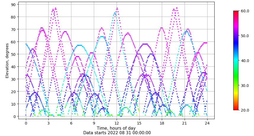
Time-elevation plot for station SALA. Signal to Noise S1C Data file SALA00ESP_R_2022243.xtr
