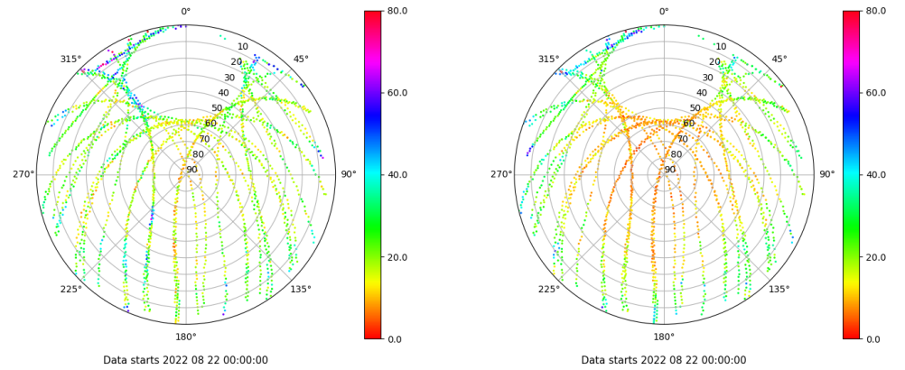
Skyplot for station SALA. Parameter M1C Data file SALA00ESP_R_2022234.xtr Skyplot for station SALA. Parameter M2P Data file SALA00ESP_R_2022234.xtr
