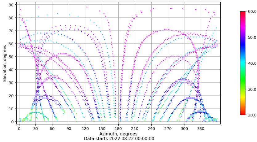
Azimuth-elevation plot for station SALA. Signal to Noise S1C Data file SALA00ESP_R_2022234.xtr
