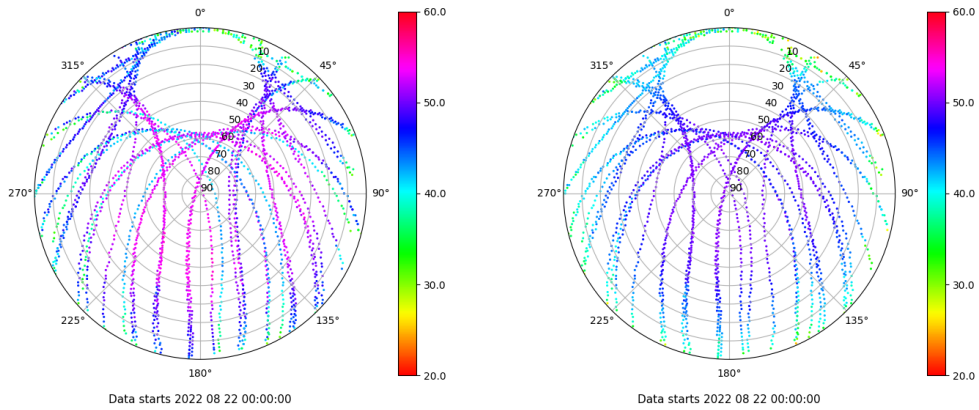
Skyplot for station SALA. Signal to Noise S1C Data file SALA00ESP_R_2022234.xtr Skyplot for station SALA. Signal to Noise S2P Data file SALA00ESP_R_2022234.xtr
