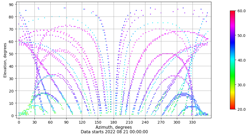
Azimuth-elevation plot for station SALA. Signal to Noise S1C Data file SALA00ESP_R_2022233.xtr
