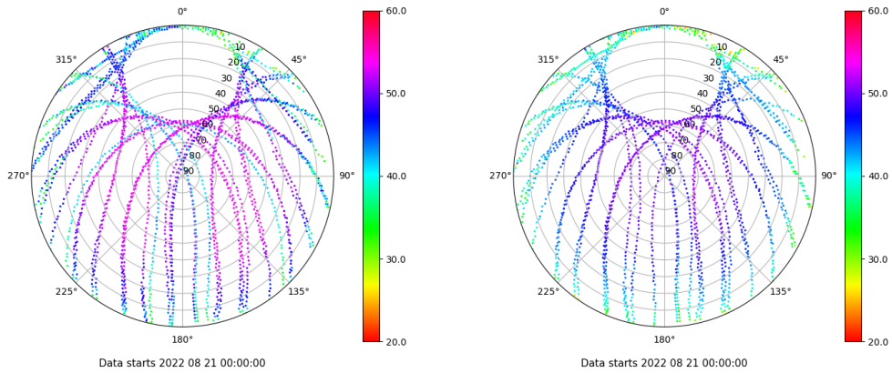
Skyplot for station SALA. Signal to Noise S1C Data file SALA00ESP_R_2022233.xtr Skyplot for station SALA. Signal to Noise S2P Data file SALA00ESP_R_2022233.xtr
