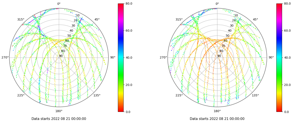
Skyplot for station SALA. Parameter M1C Data file SALA00ESP_R_2022233.xtr Skyplot for station SALA. Parameter M2P Data file SALA00ESP_R_2022233.xtr
