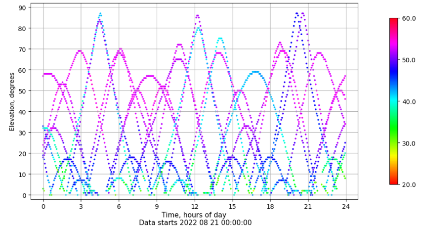
Time-elevation plot for station SALA. Signal to Noise S1C Data file SALA00ESP_R_2022233.xtr
