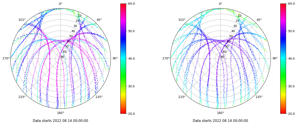
Skyplot for station SALA. Signal to Noise S1C Data file SALA00ESP_R_20222226.xtr Skyplot for station SALA. Signal to Noise S2P Data file SALA00ESP_R_20222226.xtr
