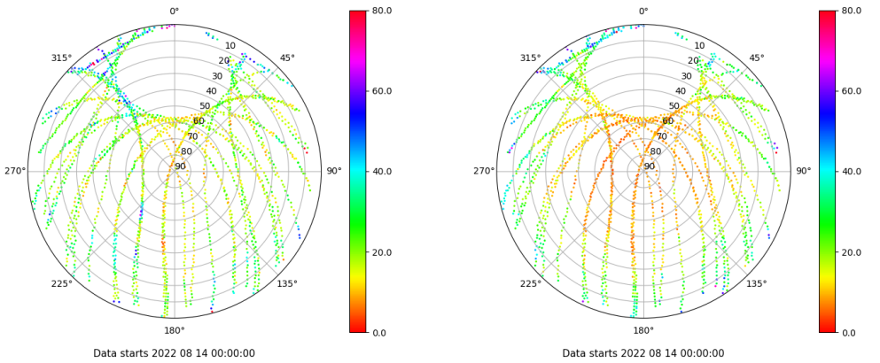
Skyplot for station SALA. Parameter M1C Data file SALA00ESP_R_20222226.xtr Skyplot for station SALA. Parameter M2P Data file SALA00ESP_R_20222226.xtr
