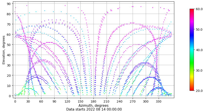
Azimuth-elevation plot for station SALA. Signal to Noise S1C Data file SALA00ESP_R_20222226.xtr
