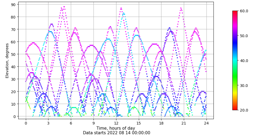
Time-elevation plot for station SALA. Signal to Noise S1C Data file SALA00ESP_R_20222226.xtr
