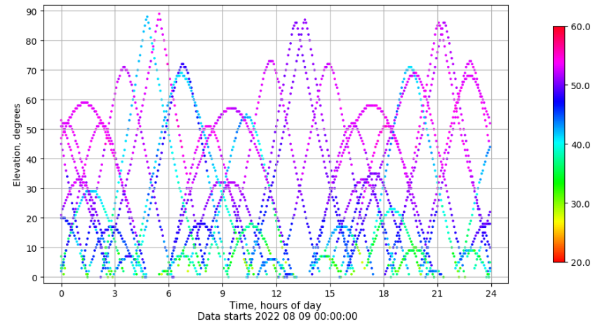
Time-elevation plot for station SALA. Signal to Noise S1C Data file SALA00ESP_R_2022221.xtr
