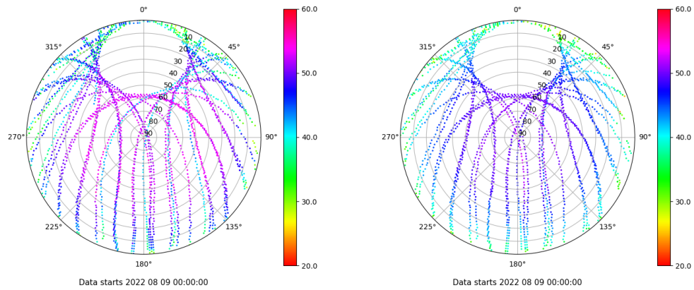
Skyplot for station SALA. Signal to Noise S1C Data file SALA00ESP_R_2022221.xtr Skyplot for station SALA. Signal to Noise S2P Data file SALA00ESP_R_2022221.xtr
