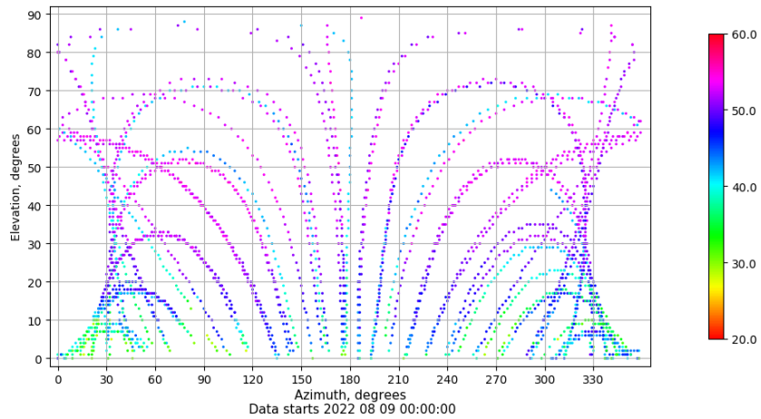
Azimuth-elevation plot for station SALA. Signal to Noise S1C Data file SALA00ESP_R_2022221.xtr
