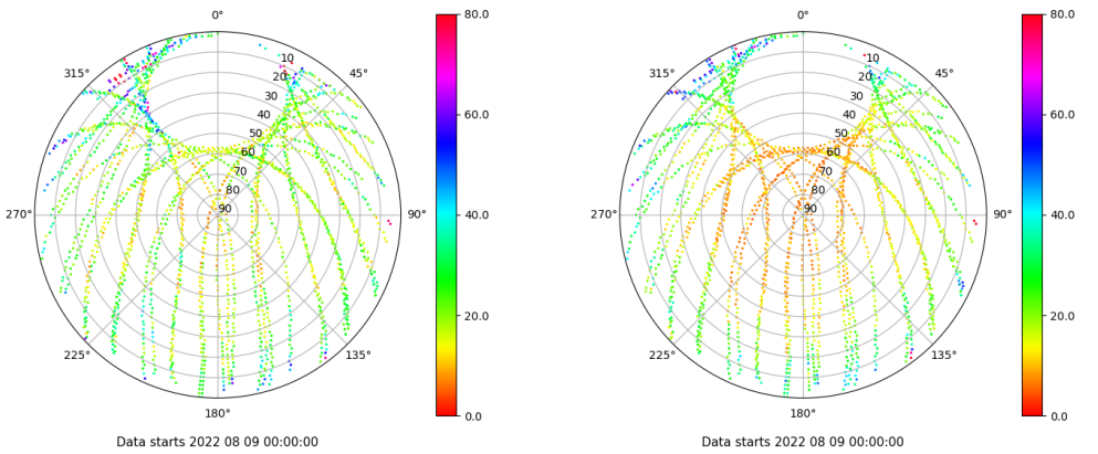
Skyplot for station SALA. Parameter M1C Data file SALA00ESP_R_2022221.xtr Skyplot for station SALA. Parameter M2P Data file SALA00ESP_R_2022221.xtr
