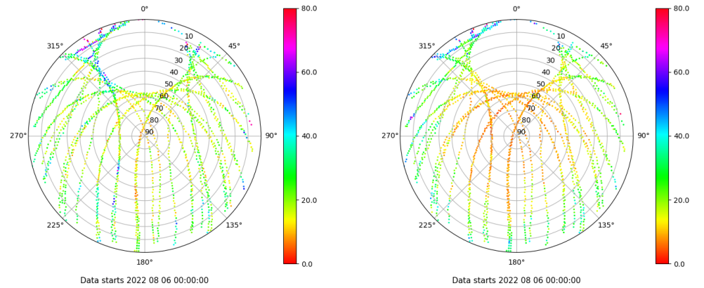
Skyplot for station SALA. Parameter M1C Data file SALA00ESP_R_2022218.xtr Skyplot for station SALA. Parameter M2P Data file SALA00ESP_R_2022218.xtr
