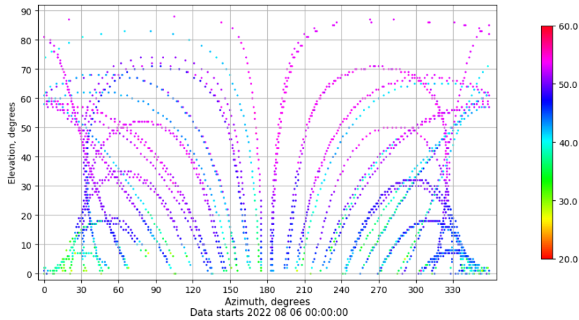
Azimuth-elevation plot for station SALA. Signal to Noise S1C Data file SALA00ESP_R_2022218.xtr
