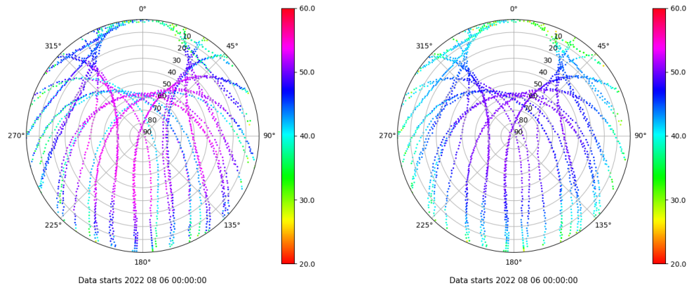
Skyplot for station SALA. Signal to Noise S1C Data file SALA00ESP_R_2022218.xtr Skyplot for station SALA. Signal to Noise S2P Data file SALA00ESP_R_2022218.xtr
