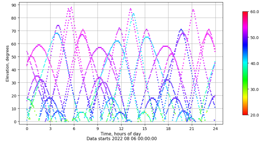
Time-elevation plot for station SALA. Signal to Noise S1C Data file SALA00ESP_R_2022218.xtr
