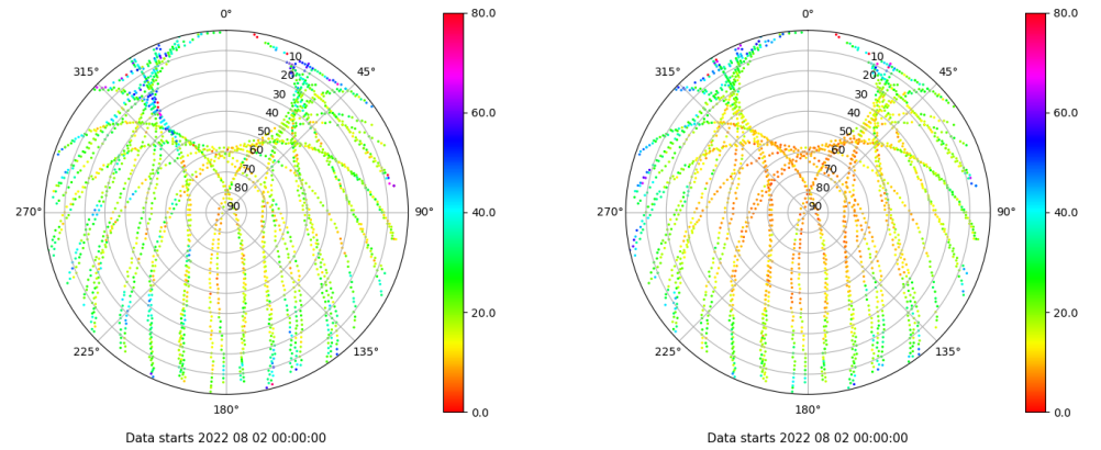
Skyplot for station SALA. Parameter M1C Data file SALA00ESP_R_2022214.xtr Skyplot for station SALA. Parameter M2P Data file SALA00ESP_R_2022214.xtr
