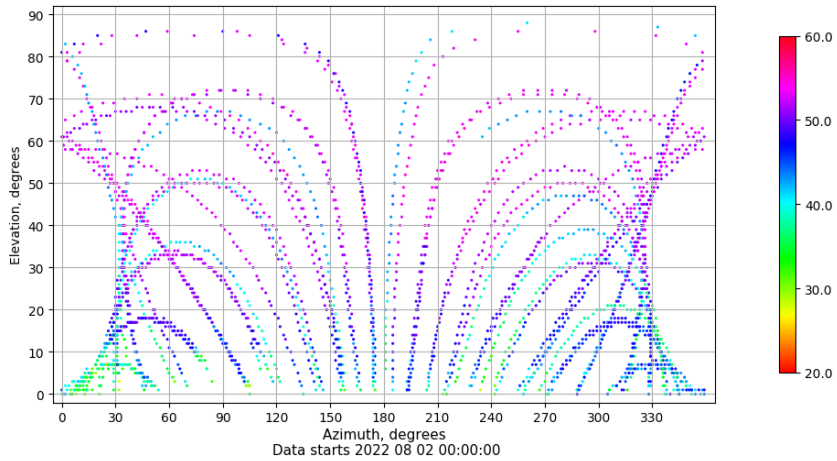
Azimuth-elevation plot for station SALA. Signal to Noise S1C Data file SALA00ESP_R_2022214.xtr
