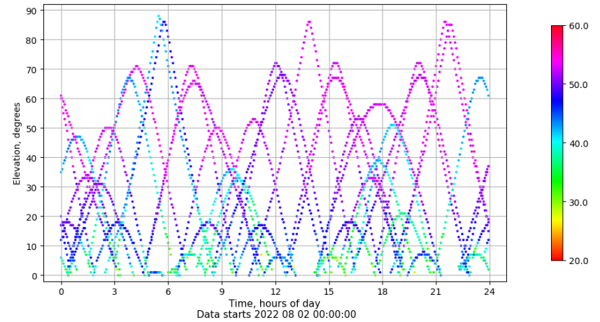
Time-elevation plot for station SALA. Signal to Noise S1C Data file SALA00ESP_R_2022214.xtr
