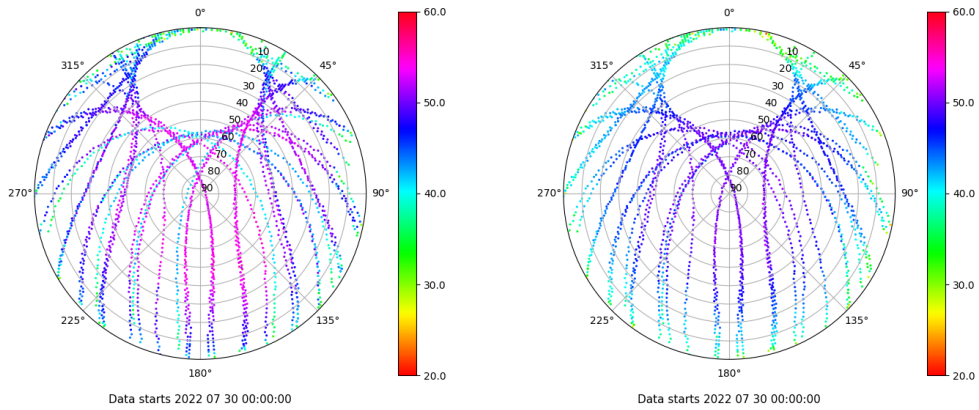
Skyplot for station SALA. Signal to Noise S1C Data file SALA00ESP_R_2022211.xtr Skyplot for station SALA. Signal to Noise S2P Data file SALA00ESP_R_2022211.xtr
