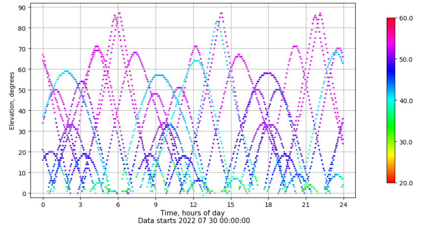
Time-elevation plot for station SALA. Signal to Noise S1C Data file SALA00ESP_R_2022211.xtr
