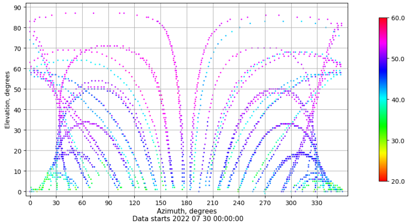
Azimuth-elevation plot for station SALA. Signal to Noise S1C Data file SALA00ESP_R_2022211.xtr
