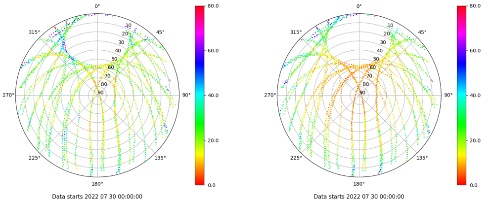
Skyplot for station SALA. Parameter M1C Data file SALA00ESP_R_2022211.xtr Skyplot for station SALA. Parameter M2P Data file SALA00ESP_R_2022211.xtr
