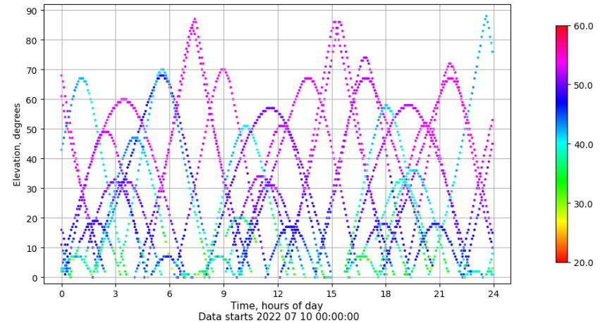
Time-elevation plot for station SALA. Signal to Noise S1C Data file SALA00ESP_R_2022191.xtr
