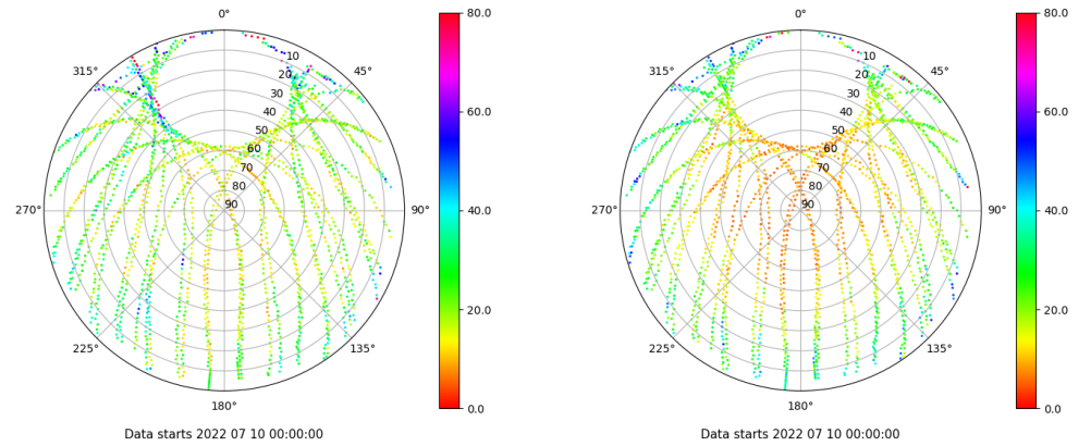
Skyplot for station SALA. Parameter M1C Data file SALA00ESP_R_2022191.xtr Skyplot for station SALA. Parameter M2P Data file SALA00ESP_R_2022191.xtr
