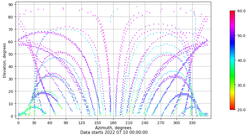
Azimuth-elevation plot for station SALA. Signal to Noise S1C Data file SALA00ESP_R_2022191.xtr
