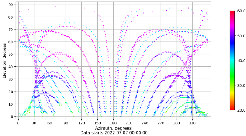
Azimuth-elevation plot for station SALA. Signal to Noise S1C Data file SALA00ESP_R_2022188.xtr
