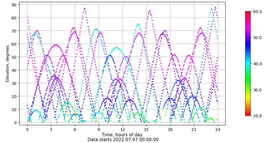
Time-elevation plot for station SALA. Signal to Noise S1C Data file SALA00ESP_R_2022188.xtr
