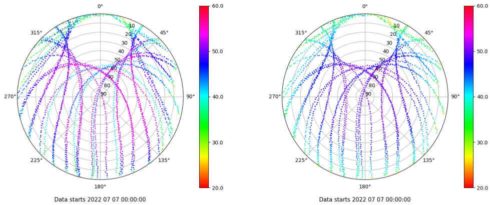
Skyplot for station SALA. Signal to Noise S1C Data file SALA00ESP_R_2022188.xtr Skyplot for station SALA. Signal to Noise S2P Data file SALA00ESP_R_2022188.xtr
