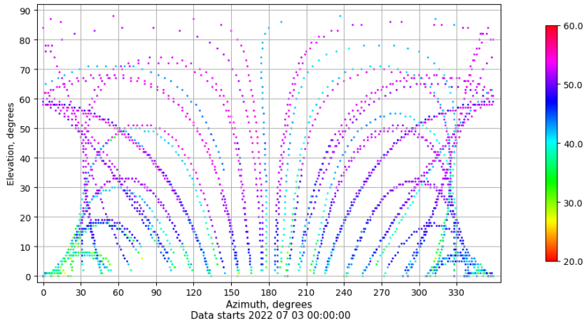
Azimuth-elevation plot for station SALA. Signal to Noise S1C Data file SALA00ESP_R_2022184.xtr
