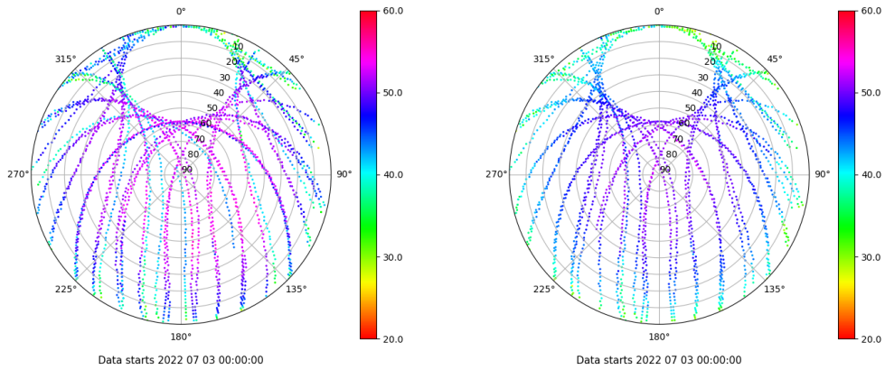
Skyplot for station SALA. Signal to Noise S1C Data file SALA00ESP_R_2022184.xtr Skyplot for station SALA. Signal to Noise S2P Data file SALA00ESP_R_2022184.xtr
