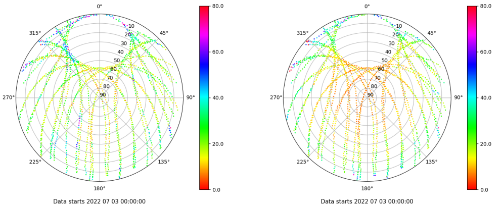
Skyplot for station SALA. Parameter M1C Data file SALA00ESP_R_2022184.xtr Skyplot for station SALA. Parameter M2P Data file SALA00ESP_R_2022184.xtr
