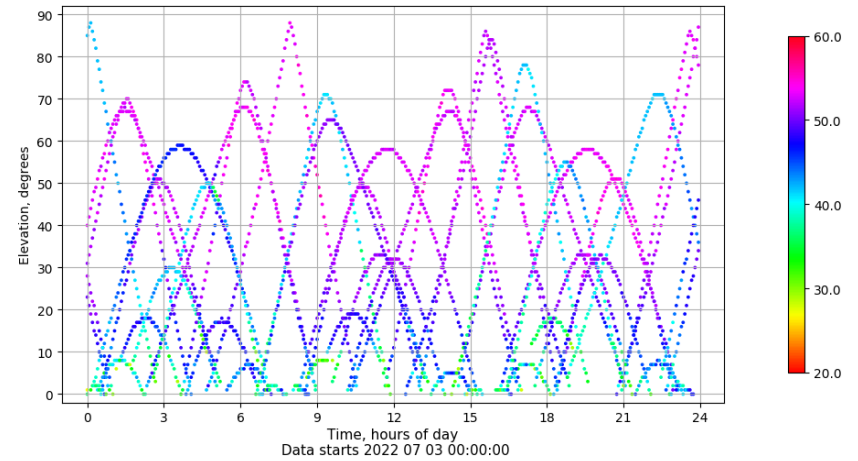
Time-elevation plot for station SALA. Signal to Noise S1C Data file SALA00ESP_R_2022184.xtr
