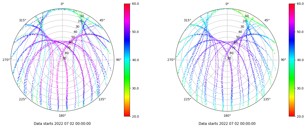
Skyplot for station SALA. Signal to Noise S1C Data file SALA00ESP_R_2022183.xtr Skyplot for station SALA. Signal to Noise S2P Data file SALA00ESP_R_2022183.xtr
