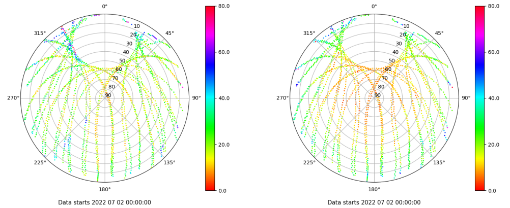
Skyplot for station SALA. Parameter M1C Data file SALA00ESP_R_2022183.xtr Skyplot for station SALA. Parameter M2P Data file SALA00ESP_R_2022183.xtr
