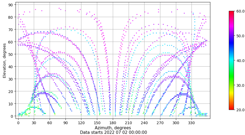
Azimuth-elevation plot for station SALA. Signal to Noise S1C Data file SALA00ESP_R_2022183.xtr
