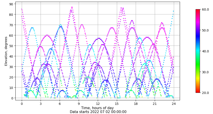
Time-elevation plot for station SALA. Signal to Noise S1C Data file SALA00ESP_R_2022183.xtr
