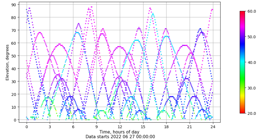
Time-elevation plot for station SALA. Signal to Noise S1C Data file SALA00ESP_R_2022178.xtr
