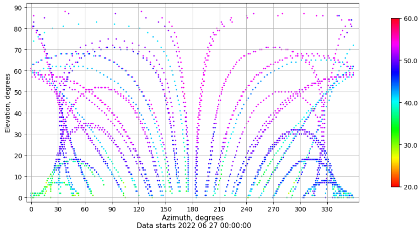
Azimuth-elevation plot for station SALA. Signal to Noise S1C Data file SALA00ESP_R_2022178.xtr
