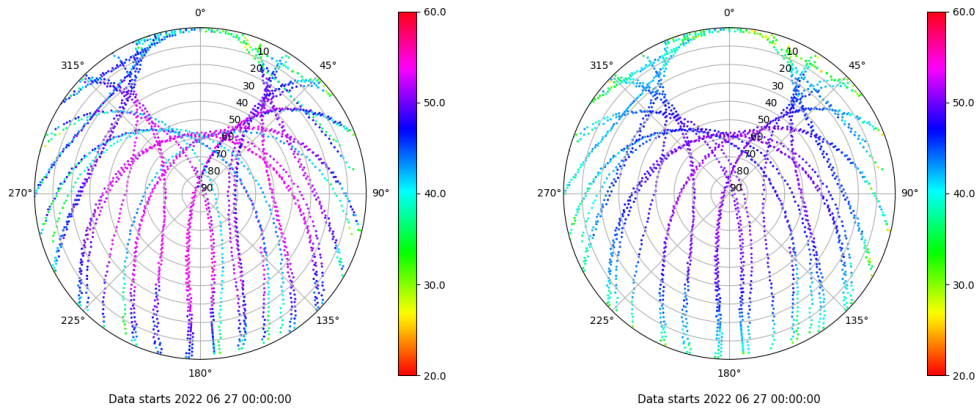
Skyplot for station SALA. Signal to Noise S1C Data file SALA00ESP_R_2022178.xtr Skyplot for station SALA. Signal to Noise S2P Data file SALA00ESP_R_2022178.xtr
