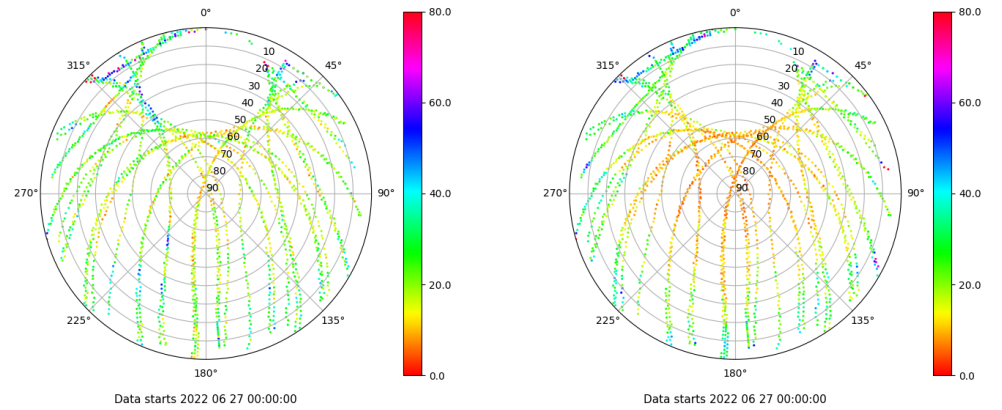
Skyplot for station SALA. Parameter M1C Data file SALA00ESP_R_2022178.xtr Skyplot for station SALA. Parameter M2P Data file SALA00ESP_R_2022178.xtr
