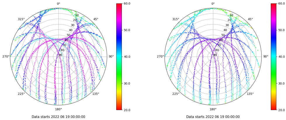
Skyplot for station SALA. Signal to Noise S1C Data file SALA00ESP_R_2022170.xtr Skyplot for station SALA. Signal to Noise S2P Data file SALA00ESP_R_2022170.xtr
