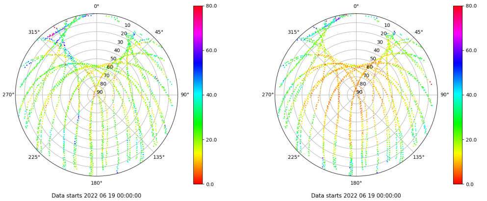
Skyplot for station SALA. Parameter M1C Data file SALA00ESP_R_2022170.xtr Skyplot for station SALA. Parameter M2P Data file SALA00ESP_R_2022170.xtr
