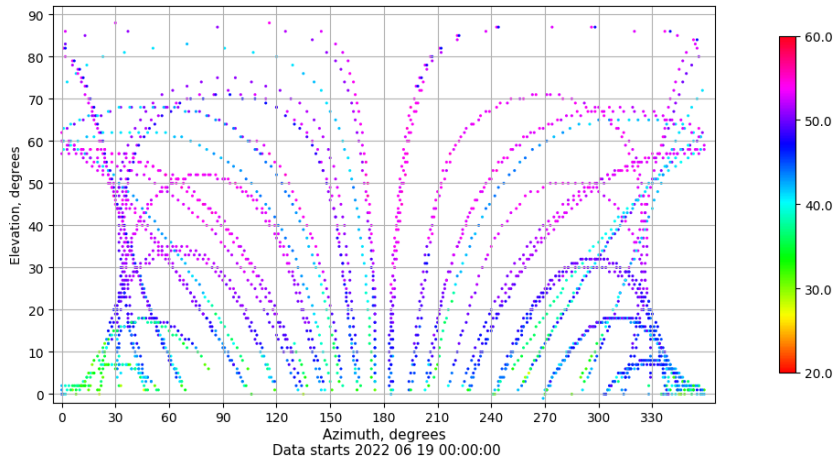
Azimuth-elevation plot for station SALA. Signal to Noise S1C Data file SALA00ESP_R_2022170.xtr
