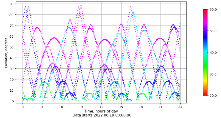
Time-elevation plot for station SALA. Signal to Noise S1C Data file SALA00ESP_R_2022170.xtr
