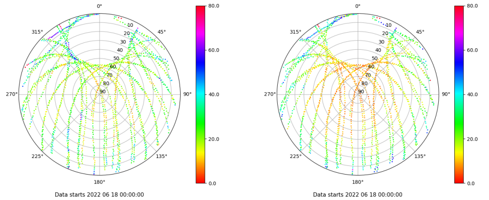
Skyplot for station SALA. Parameter M1C Data file SALA00ESP_R_2022169.xtr Skyplot for station SALA. Parameter M2P Data file SALA00ESP_R_2022169.xtr
