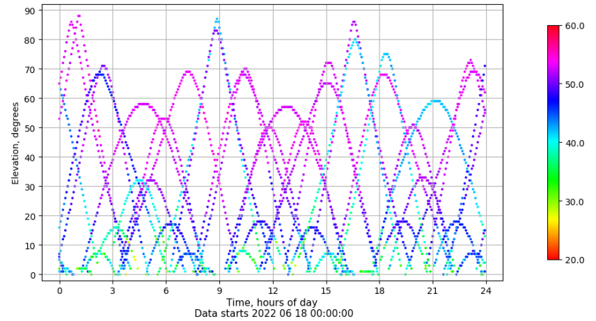
Time-elevation plot for station SALA. Signal to Noise S1C Data file SALA00ESP_R_2022169.xtr
