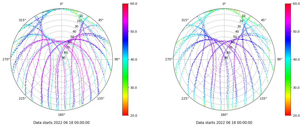
Skyplot for station SALA. Signal to Noise S1C Data file SALA00ESP_R_2022169.xtr Skyplot for station SALA. Signal to Noise S2P Data file SALA00ESP_R_2022169.xtr
