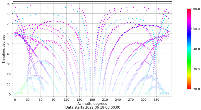
Azimuth-elevation plot for station SALA. Signal to Noise S1C Data file SALA00ESP_R_2022169.xtr
