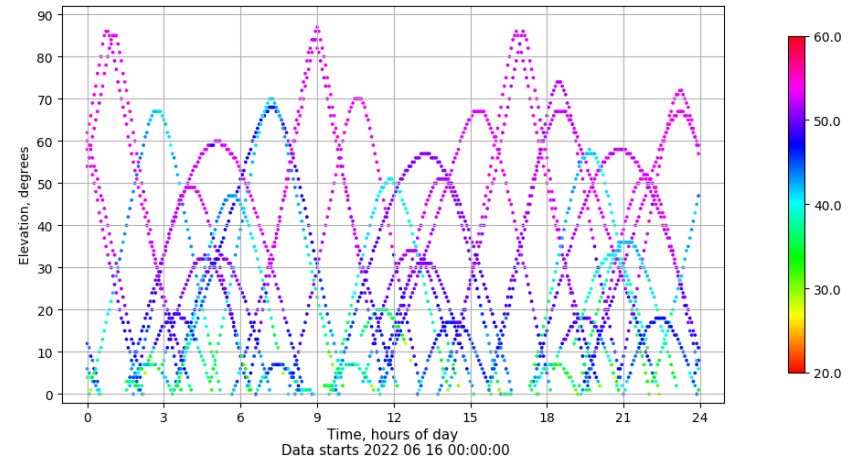
Time-elevation plot for station SALA. Signal to Noise S1C Data file SALA00ESP_R_2022167.xtr
