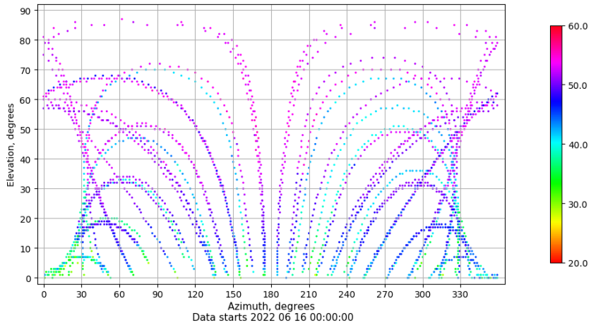
Azimuth-elevation plot for station SALA. Signal to Noise S1C Data file SALA00ESP_R_2022167.xtr
