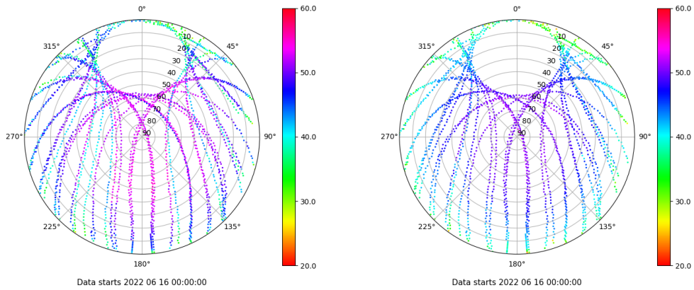
Skyplot for station SALA. Signal to Noise S1C Data file SALA00ESP_R_2022167.xtr Skyplot for station SALA. Signal to Noise S2P Data file SALA00ESP_R_2022167.xtr
