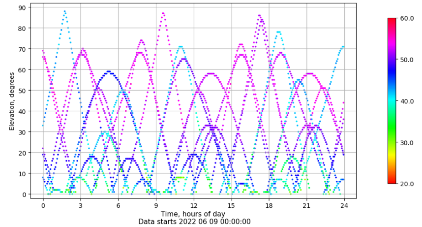
Time-elevation plot for station SALA. Signal to Noise S1C Data file SALA00ESP_R_2022160.xtr
