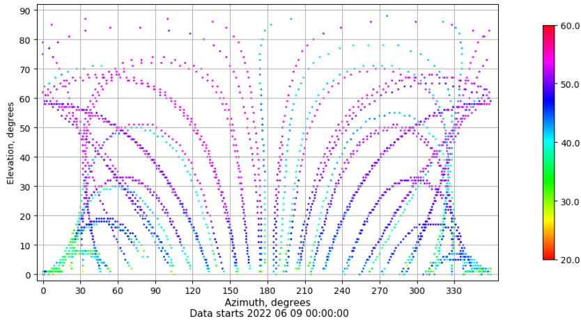
Azimuth-elevation plot for station SALA. Signal to Noise S1C Data file SALA00ESP_R_2022160.xtr
