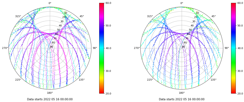
Skyplot for station SALA. Signal to Noise S1C Data file SALA00ESP_R_2022136.xtr Skyplot for station SALA. Signal to Noise S2P Data file SALA00ESP_R_2022136.xtr
