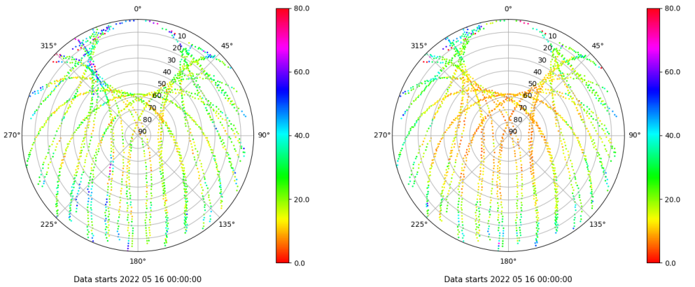
Skyplot for station SALA. Parameter M1C Data file SALA00ESP_R_2022136.xtr Skyplot for station SALA. Parameter M2P Data file SALA00ESP_R_2022136.xtr
