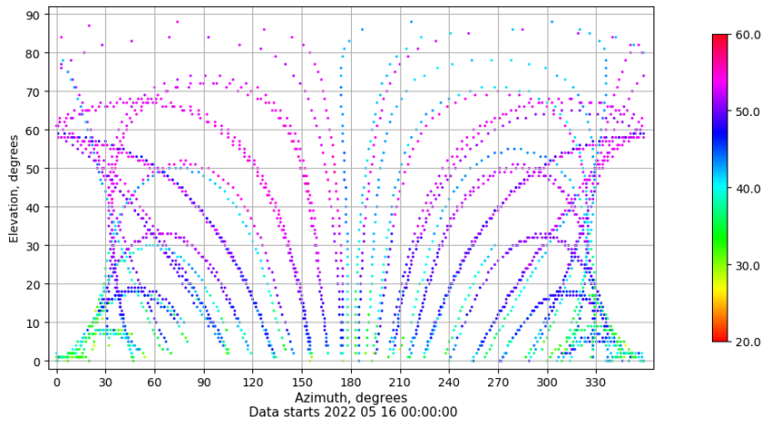
Azimuth-elevation plot for station SALA. Signal to Noise S1C Data file SALA00ESP_R_2022136.xtr
