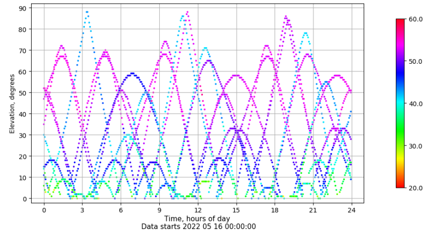
Time-elevation plot for station SALA. Signal to Noise S1C Data file SALA00ESP_R_2022136.xtr
