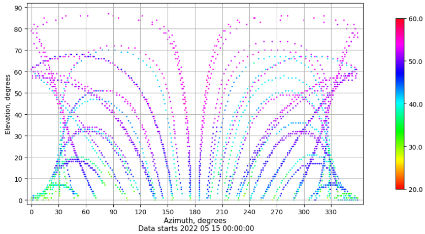
Azimuth-elevation plot for station SALA. Signal to Noise S1C Data file SALA00ESP_R_2022135.xtr
