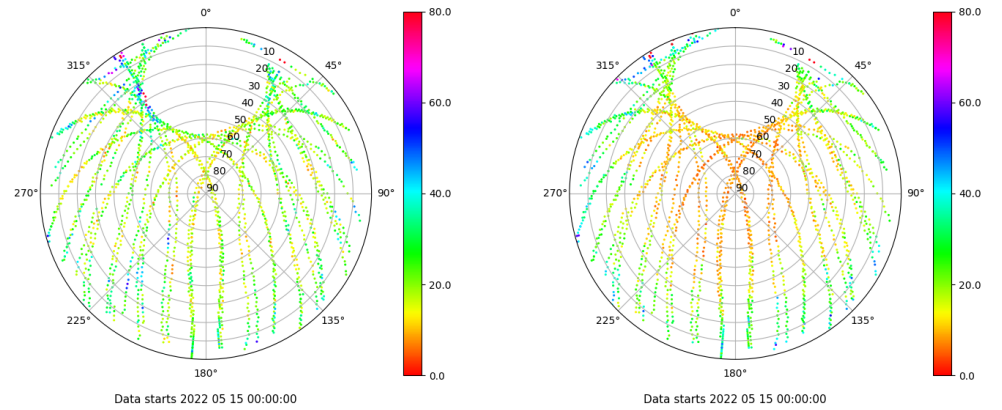
Skyplot for station SALA. Parameter M1C Data file SALA00ESP_R_2022135.xtr Skyplot for station SALA. Parameter M2P Data file SALA00ESP_R_2022135.xtr
