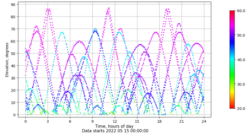
Time-elevation plot for station SALA. Signal to Noise S1C Data file SALA00ESP_R_2022135.xtr
