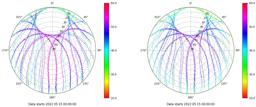
Skyplot for station SALA. Signal to Noise S1C Data file SALA00ESP_R_2022135.xtr Skyplot for station SALA. Signal to Noise S2P Data file SALA00ESP_R_2022135.xtr
