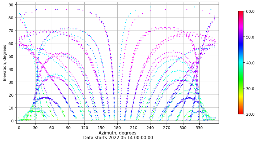
Azimuth-elevation plot for station SALA. Signal to Noise S1C Data file SALA00ESP_R_2022134.xtr
