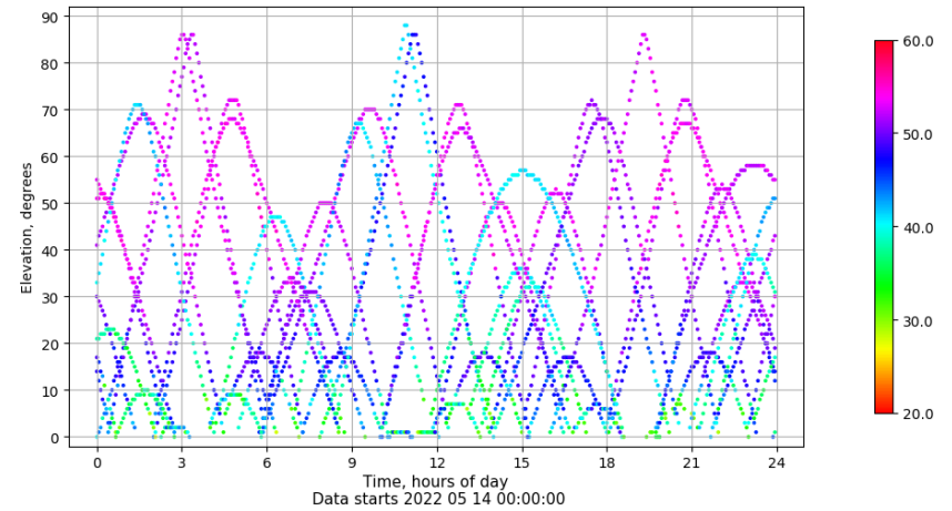
Time-elevation plot for station SALA. Signal to Noise S1C Data file SALA00ESP_R_2022134.xtr
