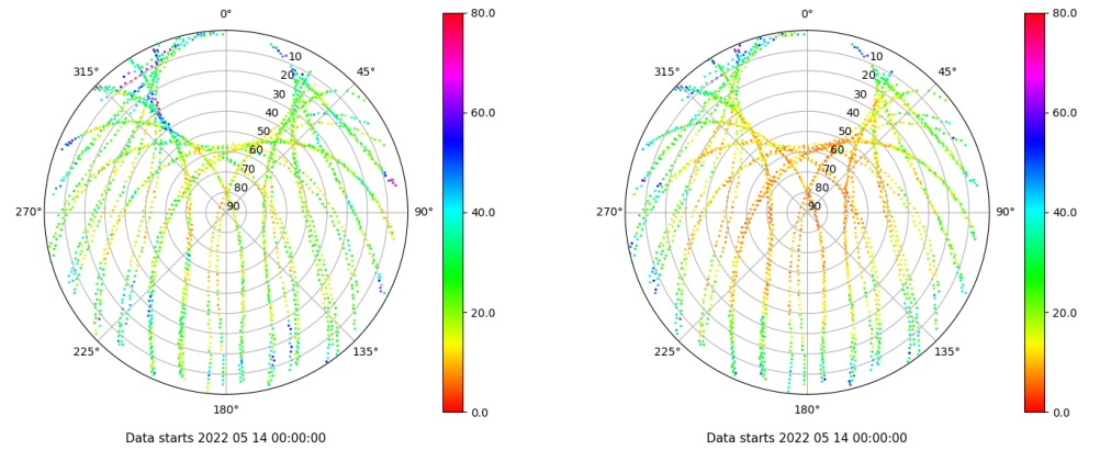
Skyplot for station SALA. Parameter M1C Data file SALA00ESP_R_2022134.xtr Skyplot for station SALA. Parameter M2P Data file SALA00ESP_R_2022134.xtr
