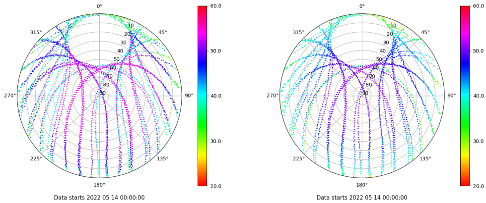
Skyplot for station SALA. Signal to Noise S1C Data file SALA00ESP_R_2022134.xtr Skyplot for station SALA. Signal to Noise S2P Data file SALA00ESP_R_2022134.xtr
