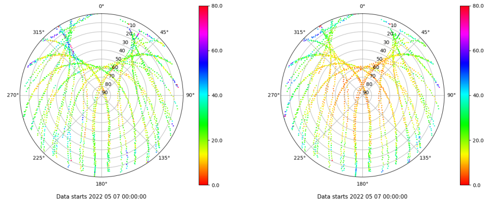
Skyplot for station SALA. Parameter M1C Data file SALA00ESP_R_2022127.xtr Skyplot for station SALA. Parameter M2P Data file SALA00ESP_R_2022127.xtr
