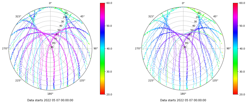
Skyplot for station SALA. Signal to Noise S1C Data file SALA00ESP_R_2022127.xtr Skyplot for station SALA. Signal to Noise S2P Data file SALA00ESP_R_2022127.xtr
