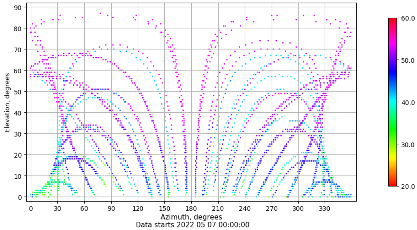
Azimuth-elevation plot for station SALA. Signal to Noise S1C Data file SALA00ESP_R_2022127.xtr
