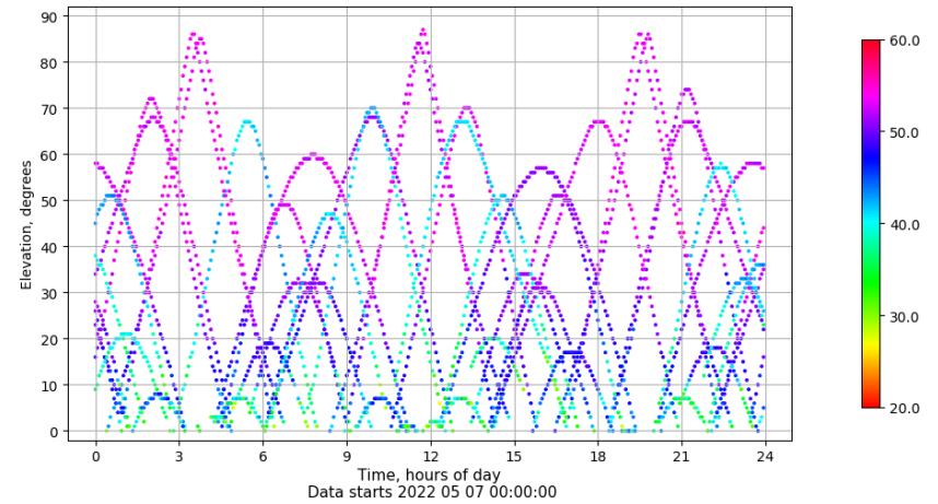
Time-elevation plot for station SALA. Signal to Noise S1C Data file SALA00ESP_R_2022127.xtr
