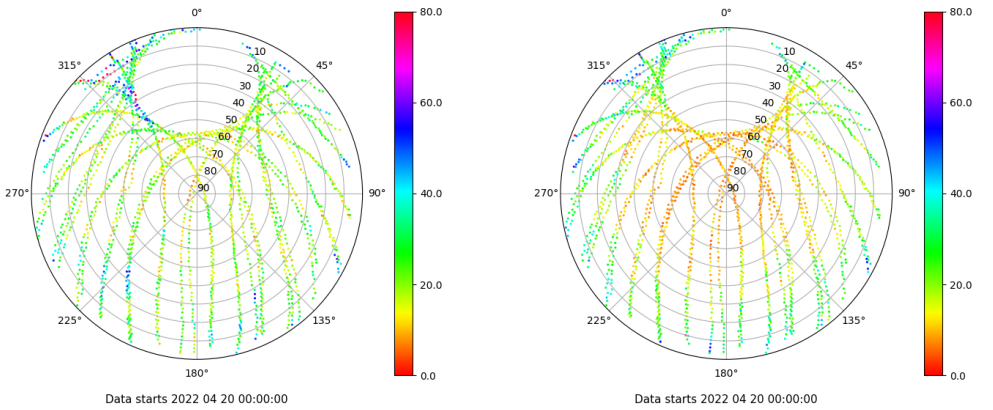
Skyplot for station SALA. Parameter M1C Data file SALA00ESP_R_2022110.xtr Skyplot for station SALA. Parameter M2P Data file SALA00ESP_R_2022110.xtr
