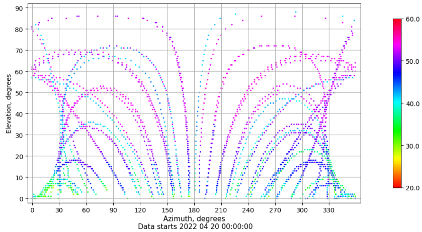
Azimuth-elevation plot for station SALA. Signal to Noise S1C Data file SALA00ESP_R_2022110.xtr
