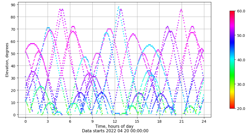
Time-elevation plot for station SALA. Signal to Noise S1C Data file SALA00ESP_R_2022110.xtr
