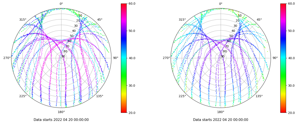
Skyplot for station SALA. Signal to Noise S1C Data file SALA00ESP_R_2022110.xtr Skyplot for station SALA. Signal to Noise S2P Data file SALA00ESP_R_2022110.xtr
