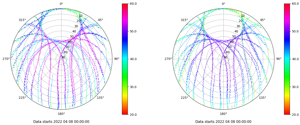
Skyplot for station SALA. Signal to Noise S1C Data file SALA00ESP_R_2022098.xtr Skyplot for station SALA. Signal to Noise S2P Data file SALA00ESP_R_2022098.xtr
