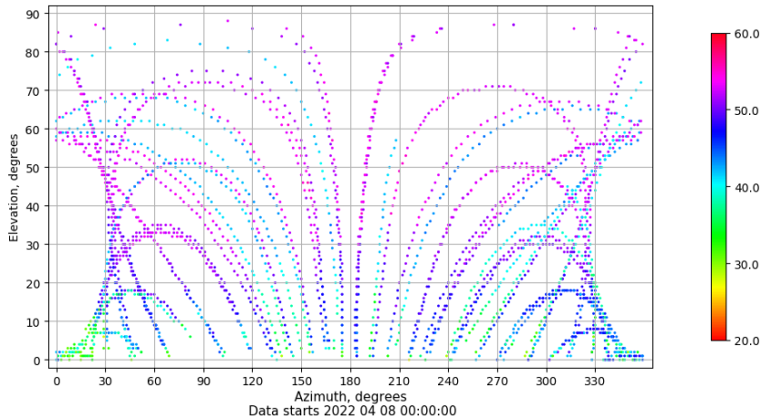
Azimuth-elevation plot for station SALA. Signal to Noise S1C Data file SALA00ESP_R_2022098.xtr
