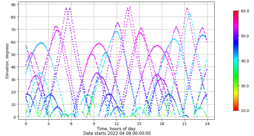
Time-elevation plot for station SALA. Signal to Noise S1C Data file SALA00ESP_R_2022098.xtr
