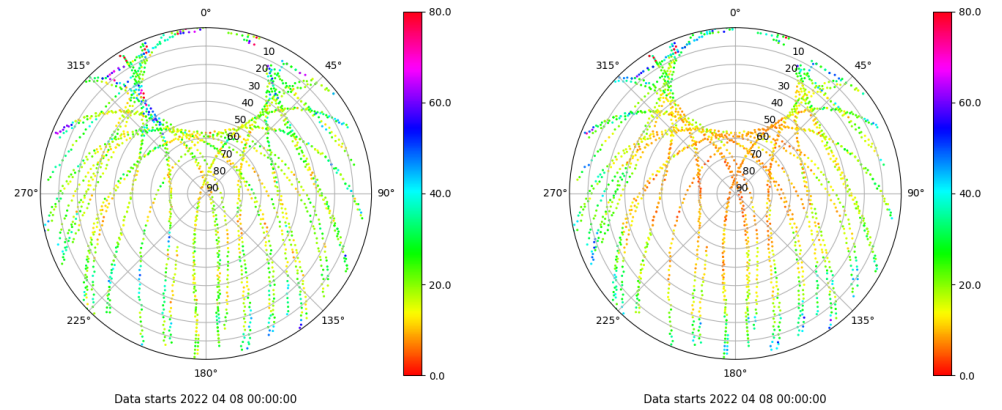
Skyplot for station SALA. Parameter M1C Data file SALA00ESP_R_2022098.xtr Skyplot for station SALA. Parameter M2P Data file SALA00ESP_R_2022098.xtr
