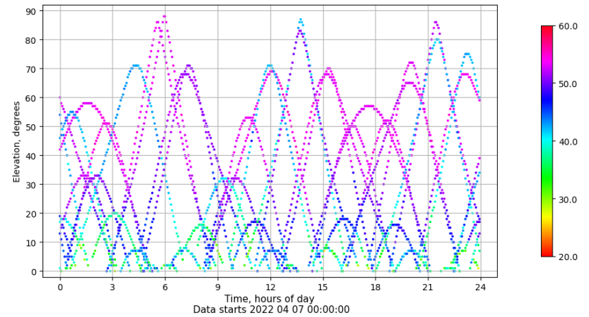
Time-elevation plot for station SALA. Signal to Noise S1C Data file SALA00ESP_R_2022097.xtr
