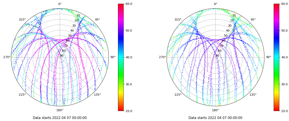
Skyplot for station SALA. Signal to Noise S1C Data file SALA00ESP_R_2022097.xtr Skyplot for station SALA. Signal to Noise S2P Data file SALA00ESP_R_2022097.xtr
