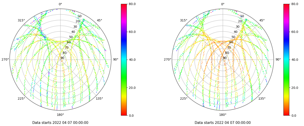
Skyplot for station SALA. Parameter M1C Data file SALA00ESP_R_2022097.xtr Skyplot for station SALA. Parameter M2P Data file SALA00ESP_R_2022097.xtr
