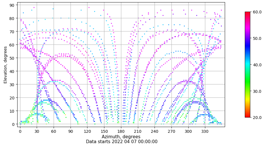
Azimuth-elevation plot for station SALA. Signal to Noise S1C Data file SALA00ESP_R_2022097.xtr
