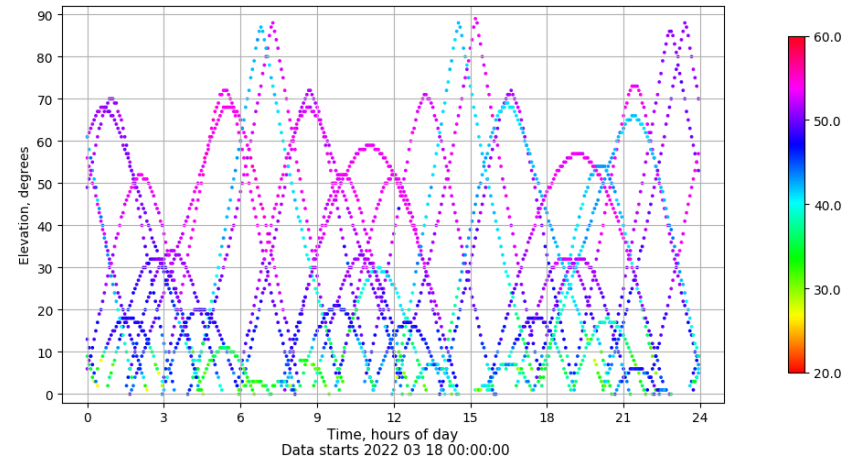
Time-elevation plot for station SALA. Signal to Noise S1C Data file SALA00ESP_R_2022077.xtr
