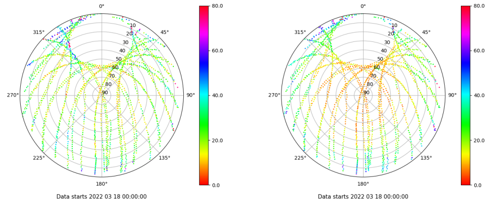
Skyplot for station SALA. Parameter M1C Data file SALA00ESP_R_2022077.xtr Skyplot for station SALA. Parameter M2P Data file SALA00ESP_R_2022077.xtr
