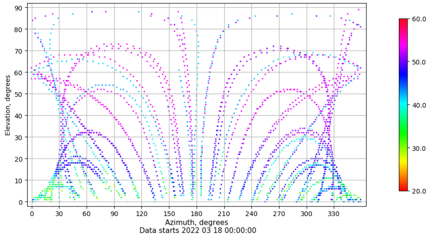
Azimuth-elevation plot for station SALA. Signal to Noise S1C Data file SALA00ESP_R_2022077.xtr
