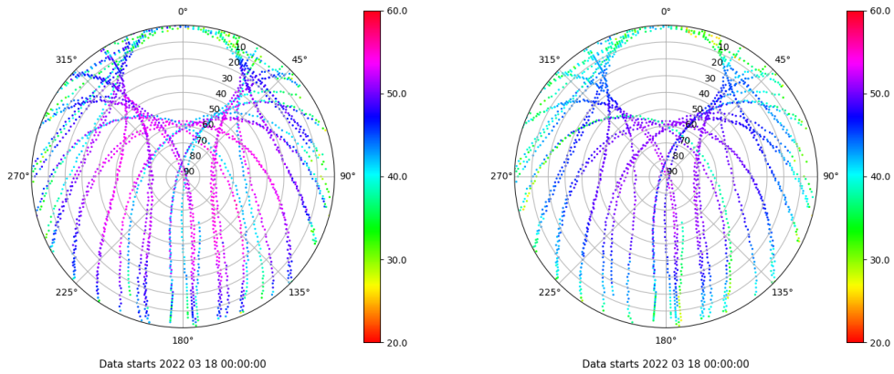
Skyplot for station SALA. Signal to Noise S1C Data file SALA00ESP_R_2022077.xtr Skyplot for station SALA. Signal to Noise S2P Data file SALA00ESP_R_2022077.xtr
