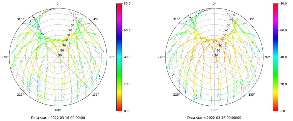
Skyplot for station SALA. Parameter M1C Data file SALA00ESP_R_2022075.xtr Skyplot for station SALA. Parameter M2P Data file SALA00ESP_R_2022075.xtr
