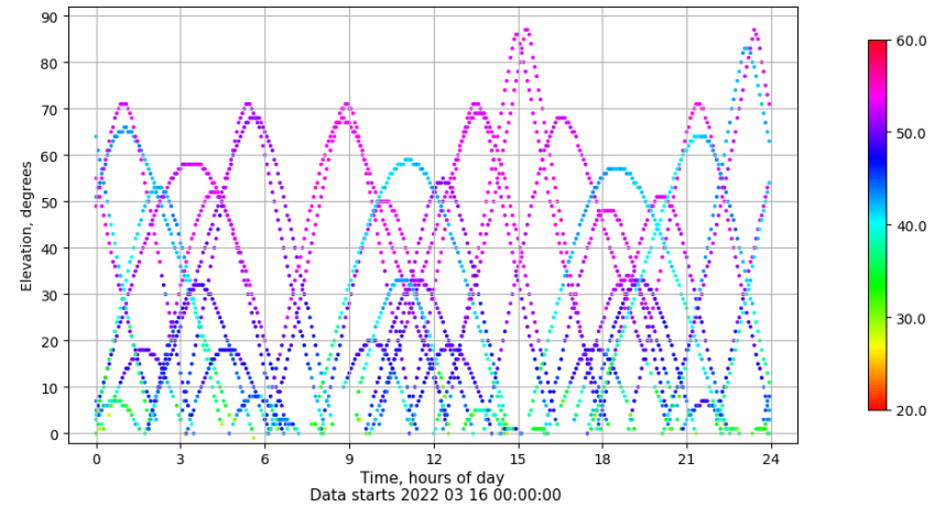
Time-elevation plot for station SALA. Signal to Noise S1C Data file SALA00ESP_R_2022075.xtr
