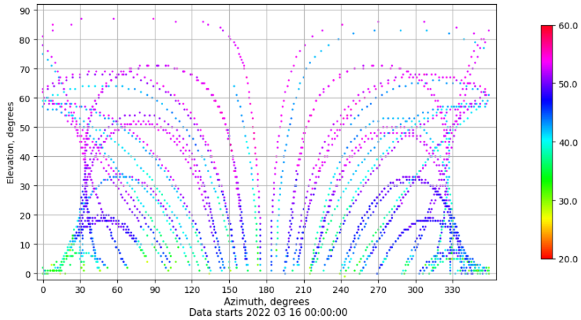
Azimuth-elevation plot for station SALA. Signal to Noise S1C Data file SALA00ESP_R_2022075.xtr
