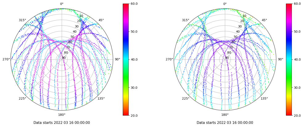
Skyplot for station SALA. Signal to Noise S1C Data file SALA00ESP_R_2022075.xtr Skyplot for station SALA. Signal to Noise S2P Data file SALA00ESP_R_2022075.xtr
